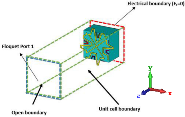
Fig. 4. Physical representation of the TZZ_{inv} absorber.
