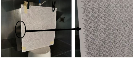
Fig. 12. Global view and detail of the ATZZ_{inv} FSS absorber printed on a 100\ \mu\text{m} -thick aramid sheet.
