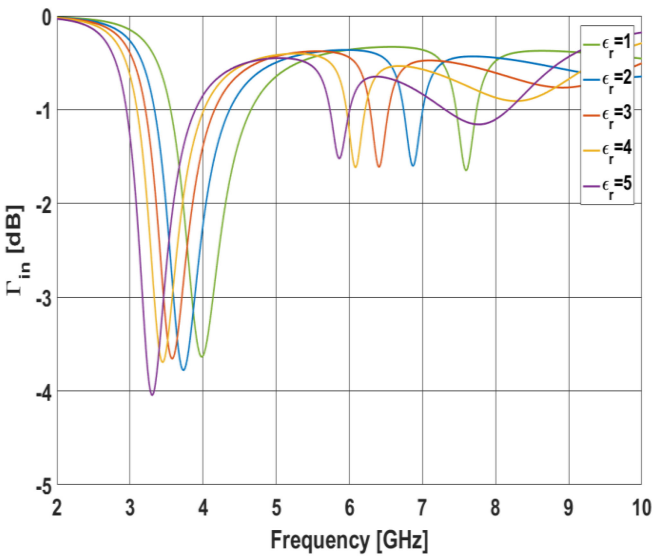
Fig. 5. Simulated reflection coefficient vs. dielectric permittivity values of a copper TZZ_{inv} pattern printed on a 4 mm-thick dielectric substrate.
