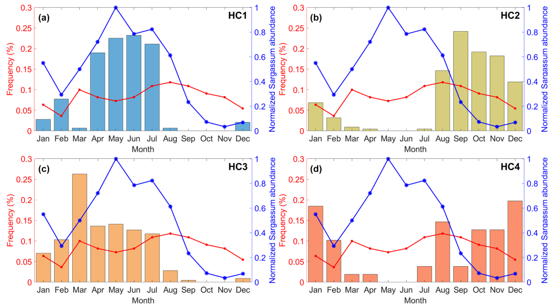
Figure 15. Monthly distribution of cluster occurrence from HYCOM outputs from 2019 to 2020 in the Lesser Antilles ( 55\text{--}66^\circ\text{W} , 8\text{--}17^\circ\text{N} ): HC1 (a), HC2 (b), HC3 (c), and HC4 (d). The red line shows the monthly distribution of Sargassum beachings on the coasts of Guadeloupe during the same period. The blue line indicates the monthly evolution of Sargassum abundance in the area 30–100 km offshore of Guadeloupe normalized on the maximum value.
