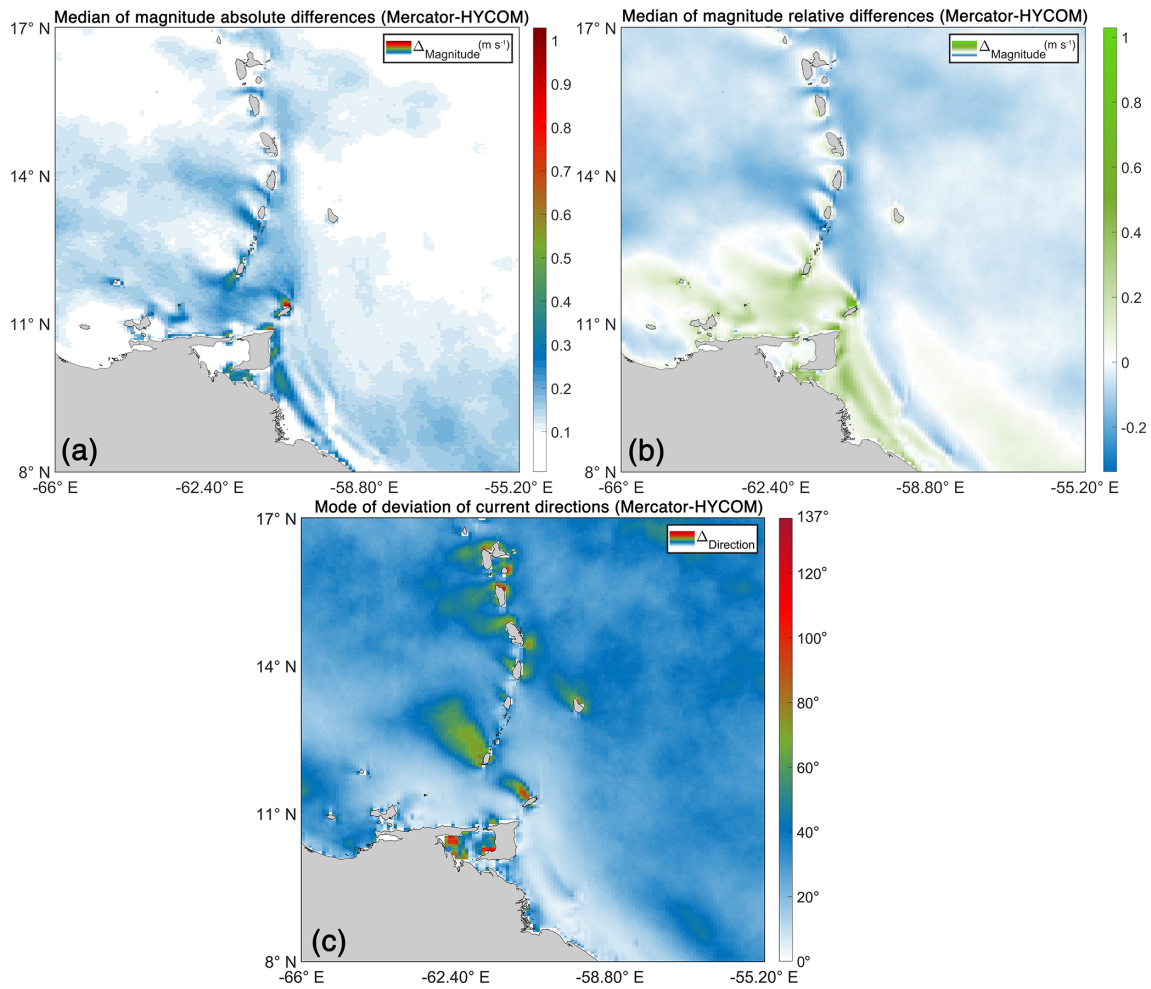
Figure 8. Comparison between Mercator and HYCOM surface currents from 2019 to 2020 on the same 0.08° grid: (a) median of magnitude absolute differences (Mercator–HYCOM) ( \text{m s}^{-1} ), (b) median of magnitude relative differences (Mercator–HYCOM) ( \text{m s}^{-1} ), and (c) mode of current direction differences (Mercator–HYCOM) (degrees).
