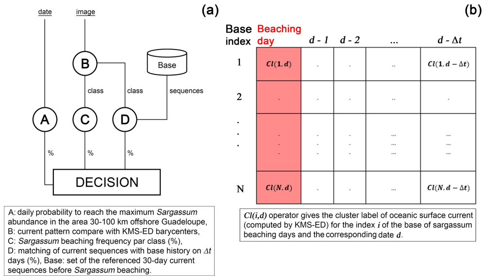
Figure 5. (a) Scheme of the decision tree classifier to predict Sargassum beaching probability. (b) Combination base of oceanic current cluster labels obtained by KMS-ED from each beaching day to Δt days before.
