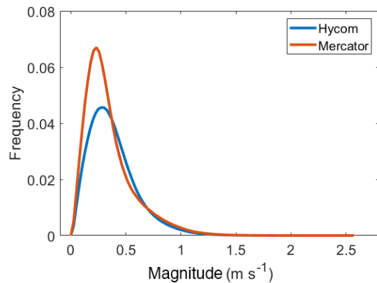
Figure 6. Distributions of oceanic surface current magnitudes including windage for both models: HYCOM (blue) and Mercator (red) datasets.
