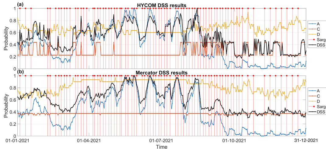
Figure 18. Decision support system (DSS) results: probability of beaching obtained per module. Daily probability to reach the maximum Sargassum abundance in the area 30–100 km offshore of Guadeloupe for module A (blue line), beaching frequency per cluster for module C (orange line), match percentage for module D (yellow line), and DSS decision (black line). Days of observed beaching on Guadeloupe coasts (red dots): HYCOM (a) and Mercator (b).
