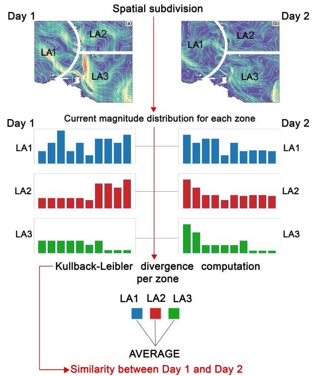
Figure 3. The schematic of the expert distance process.
