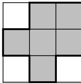
figure 2.1: a 2D polyomino
