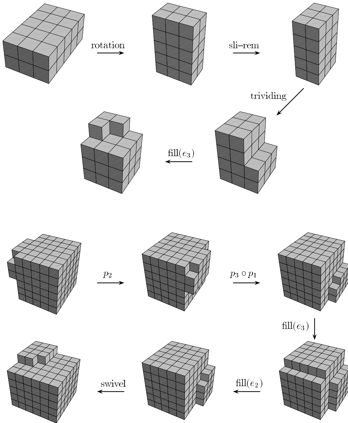
figure 3.14: two examples
