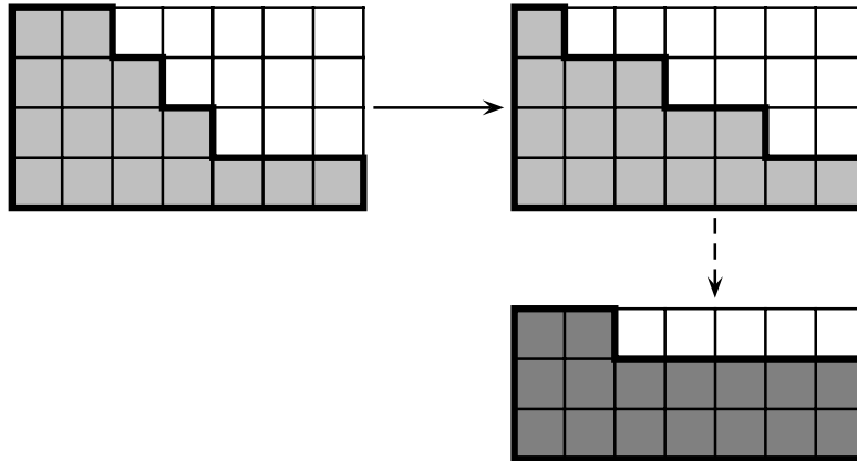
figure 2.10: filling(2 → 1)
