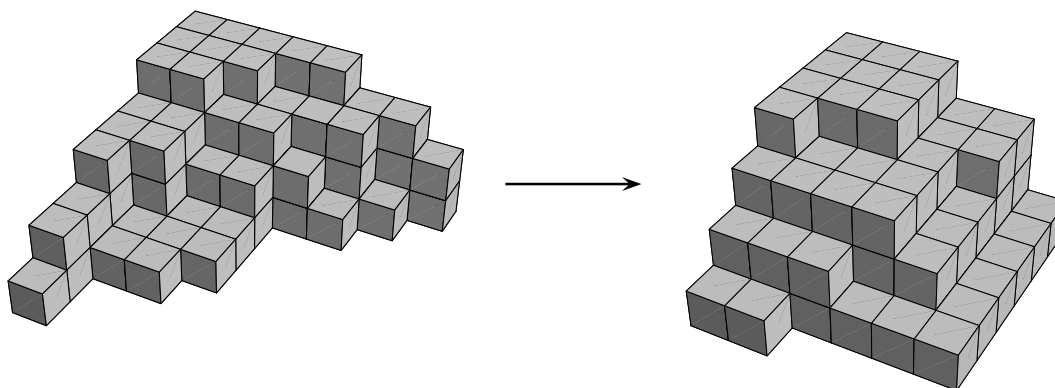
figure 3.6: slice-remodelling
