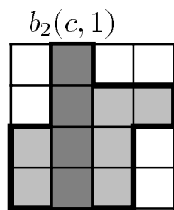
figure 2.4: a bar
