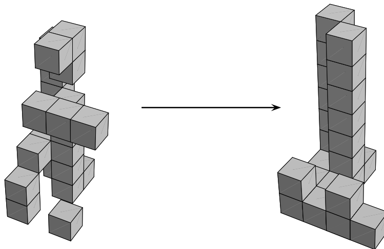
figure 3.5: projection p_3
