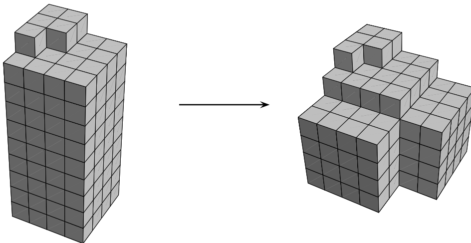
figure 3.11: trividing
