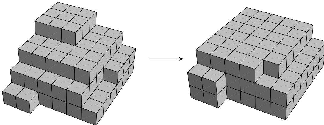
figure 3.10: filling( e_3 )
