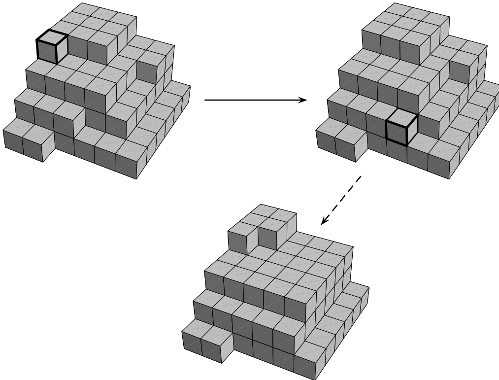
figure 3.7: cube-moving
