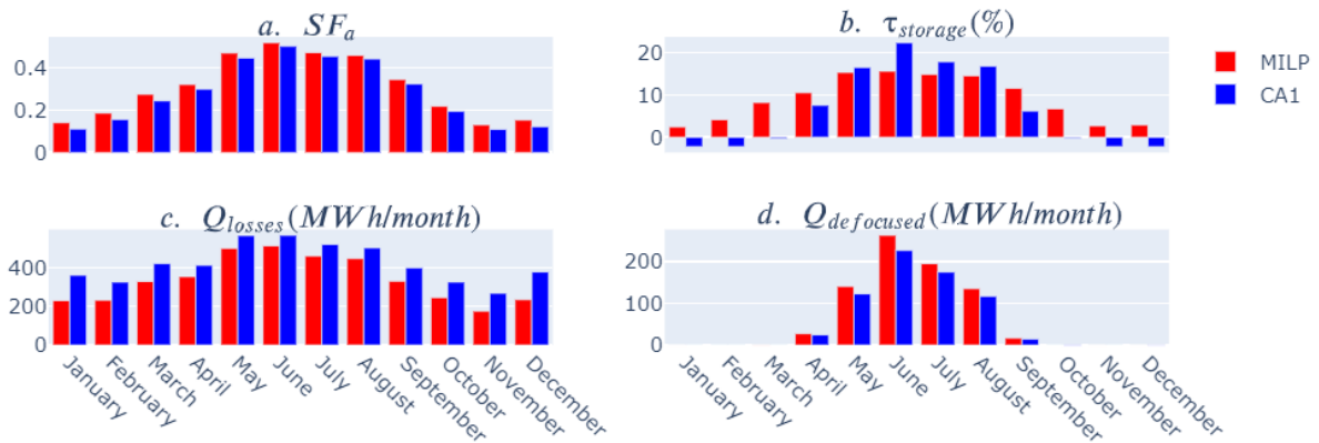
Fig. 8. Yearly metrics.
