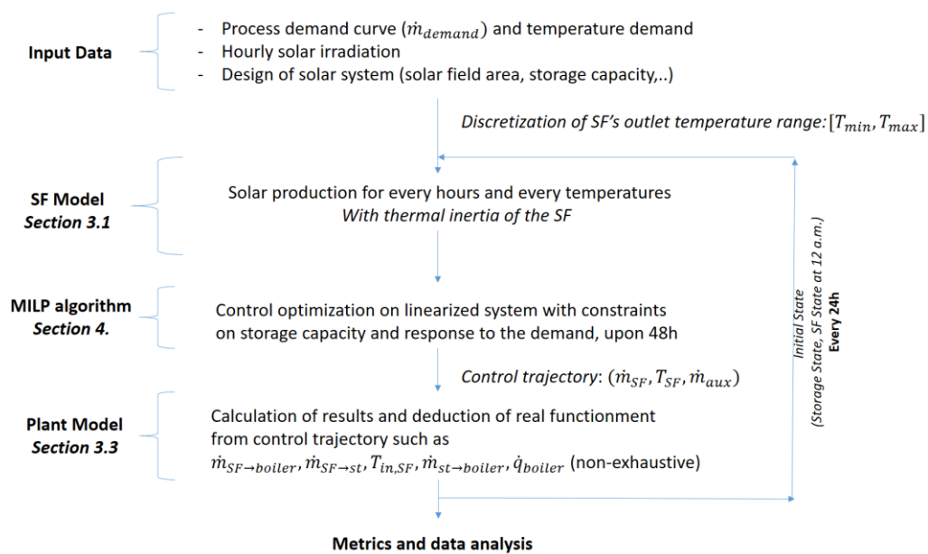
Fig. 2. Algorithm structure
