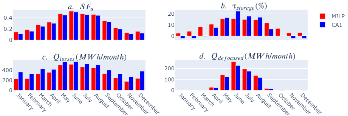
Fig. 8. Yearly metrics.
