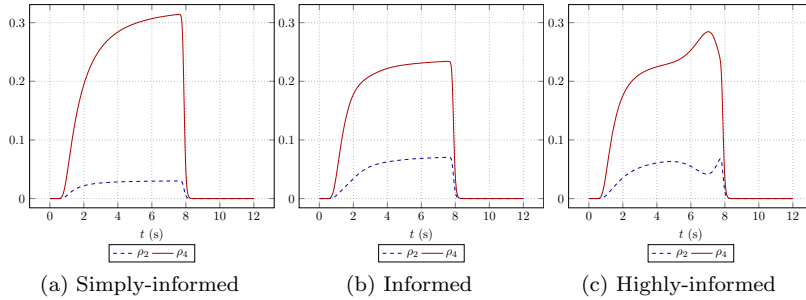
Fig. 4: Simple network with 5 roads (Fig. 2): time evolution of the density \rho_2(t, 0) and \rho_4(t, 0) at the beginning of streets 2 and 4.
