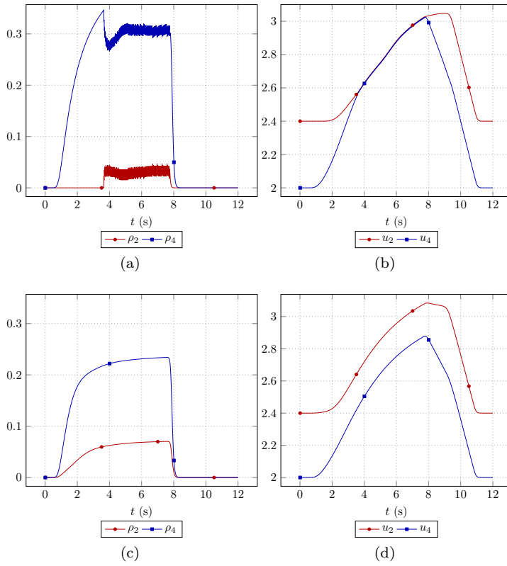
Fig. 1: Different choices of the activation function \psi on a simple informed population on the 5 roads network considered in Section 4.1. In the case of the step function \bar{\psi} (Figures (a) and (b)) the agents choosing road 2 (whose incoming density is \rho_2 ) and road 4 (represented by \rho_4 ) switch continuously between the two option of identical value function u_2, u_4 , with some oscillatory effects on the densities. In Fig. (c) and (d), the use of the smooth activation function \hat{\psi} with \epsilon = 1 prevents these effects and the agents distribute smoothly on the two paths.
