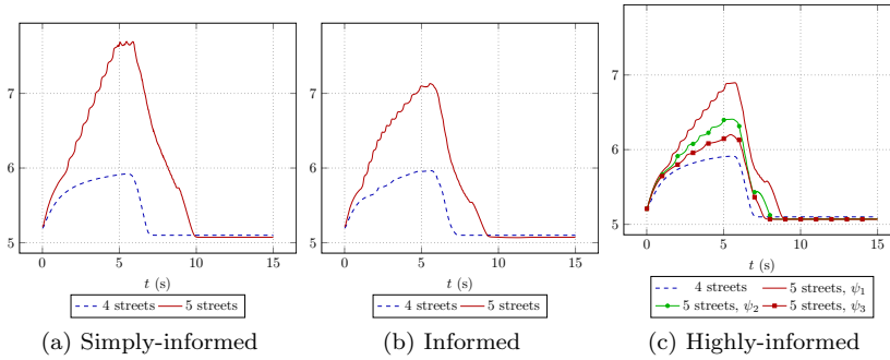
Fig. 7: Braess' network (Fig. 6): travel time TT(1, 6, t) , t \in [0, 15] for different level of information. Here \epsilon = \{1, 2, 3\}
