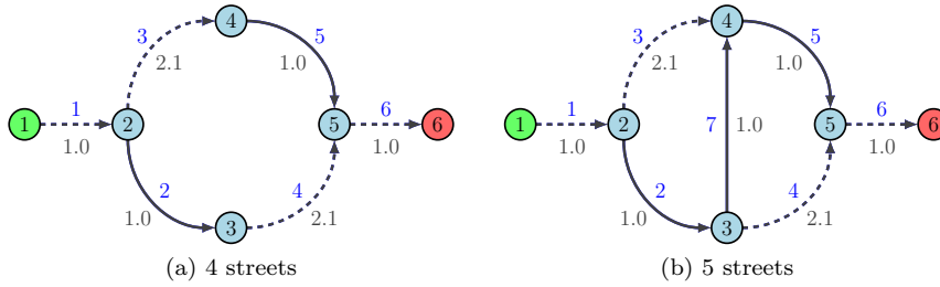
Fig. 6: Braess' paradox network: origin (green) and destination (red) junctions are enlighten; id (above) and the length (below) of the streets are reported; constant speed streets (dashed) are marked.
