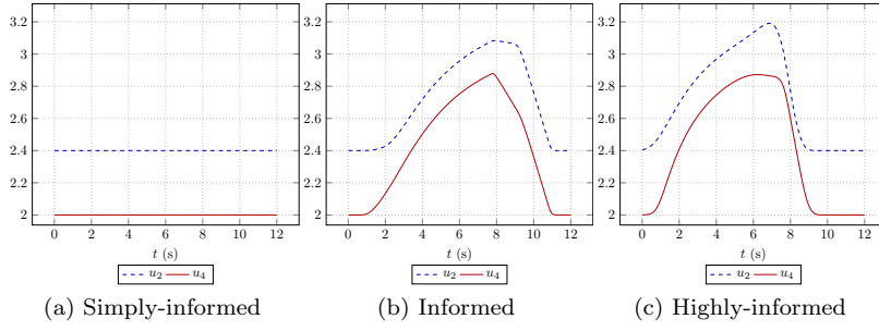
Fig. 5: Simple network with 5 roads (Fig. 2): time evolution of the costs u_2(t, 0) and u_4(t, 0) at the beginning of streets 2 and 4.
