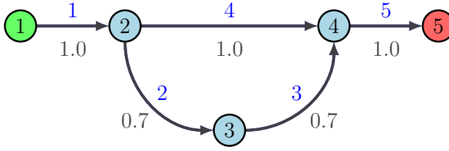
Fig. 2: Simple network with 5 roads and two possible paths to reach destination; origin (green) and destination (red) junctions are enlighten; id (above) and the length (below) of the roads are reported.
