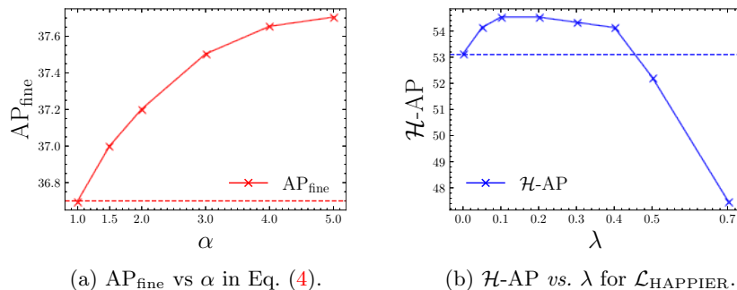
Fig. 4: Impact on Inat-base of \alpha in Eq. (4) for setting the relevance of \mathcal{H}\text{-AP} (a) and of the \lambda hyper-parameter on HAPPIER results (b).
