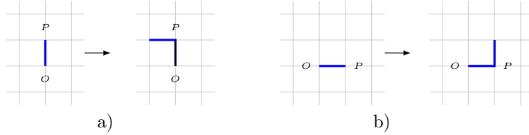
Figure 13: Split operator applied to Christoffel paths of slopes (a) \infty so that split(1) = (\bar{1}\bar{0}, 0) , and (b) 0 such that split(0) = (0\bar{1}, \bar{1}) .
