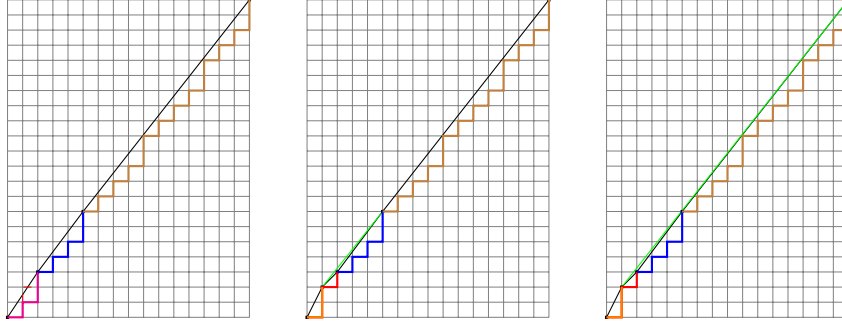
Figure 16: Procedure of insertability verification on the right with propagation: the closest upper point (1, 2) of l_i ( l_i in pink) is inserted (left); as l_{i+1} \leq R_0 ( l_{i+1} in blue and R_0 = l^- in red) is not satisfied but we have l_{i+1} = R_0 l_i , we obtain R_1 = R_0 l_{i+1} ( R_1 in green (=red+blue)) (center); as l_{i+2} \leq R_1 ( l_{i+2} in brown) is not satisfied but we have l_{i+2} = R_1^2 l_{i+1} , we obtain R_2 = R_1 l_{i+2} ( R_2 in green (=red+blue+brown)) (right).
