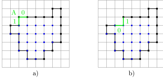
Figure 8: a) A is a point in the \mathcal{WN} -path, where its neighboring points back and forth in Bd_{\mathcal{WN}}(C) form the sub-word 10. b) Removing the point A corresponds to switching the sub-word 10 into 01, i.e applying the switch operator at the position of the point A
