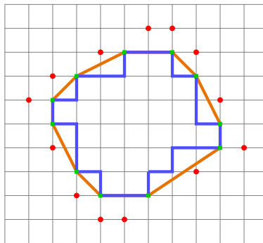
Figure 1: The green points are the removable points, which are the vertices of the convex hull of a digital convex set C . The red points are the insertable points, which some are the exterior Bézout point of each segment of the convex hull.
