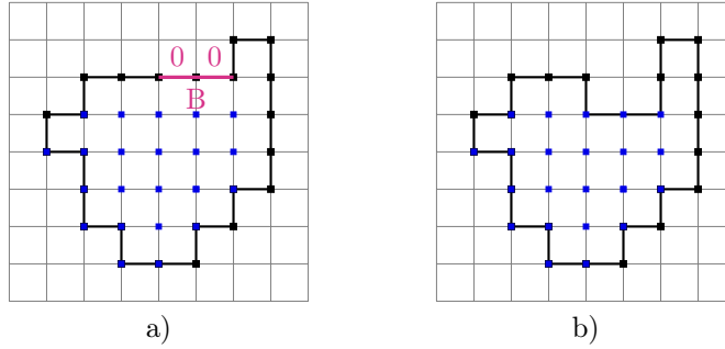
Figure 9: a) B is a point in the \mathcal{WN} -path, where its neighboring points back and forth in Bd_{\mathcal{WN}}(C) form the sub-word 00. b) The digital convexity is lost when removing the point B
