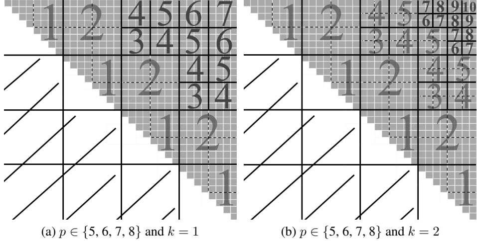
Figure 3: Four-splitting technique of the shortest path matrix for n = 32 , k \in \{1, 2\} , and p \in \{5, 6, 7, 8\} . SP is partitioned into nineteen blocks and thirty-six subblocks when k = 1 , and into twenty-eight blocks and seventy-two subblocks when k = 2
