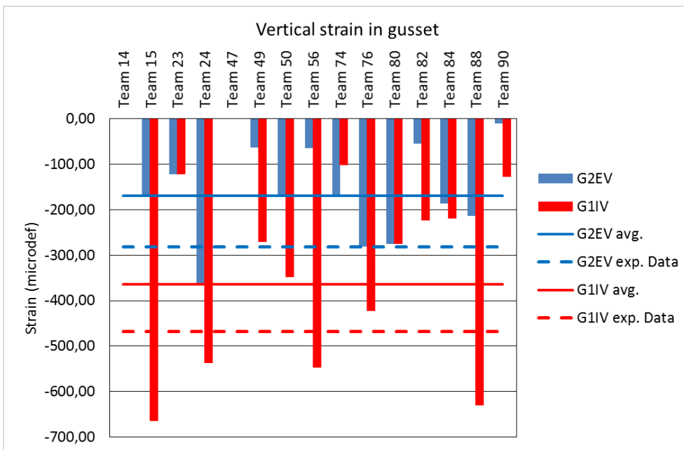
Figure 17 - Vertical ageing strains in the gusset
