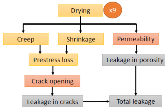
Figure 3 - Aging process of VERCORS mock-up. Grey boxes are relevant during a pressure test or an accident only. During normal operation, the pressure difference between both sides of the wall is very low.
