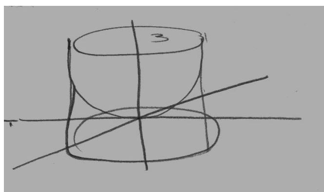
Figure 3 – A student’s view of points in R^2 that satisfy x^2 + y^2 = 1 and are assigned a height of 3.
