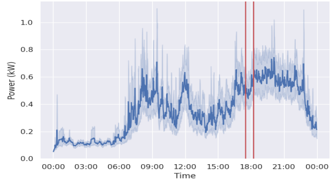
Fig. 2: Average consumption profile as provided by the ELVTF model. Our shedding scenario is simulated between 5:30 PM to 6:15 PM, between the two red bars.
