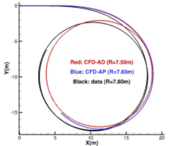
Fig.21 Trajectory of the KCS TC35 motion
