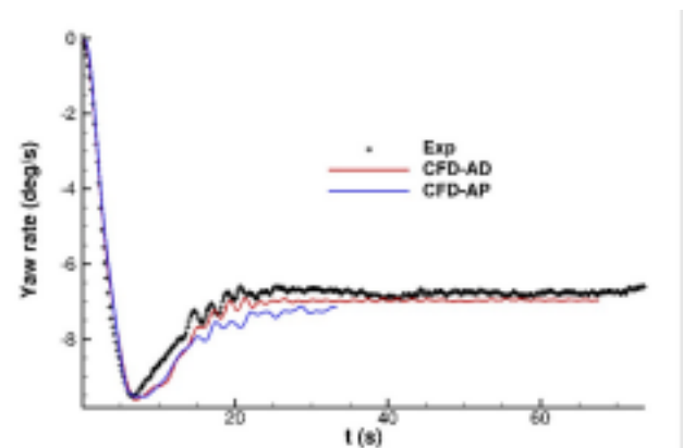
Fig.27 Time history of yaw rate for the KCS TC35 motion
