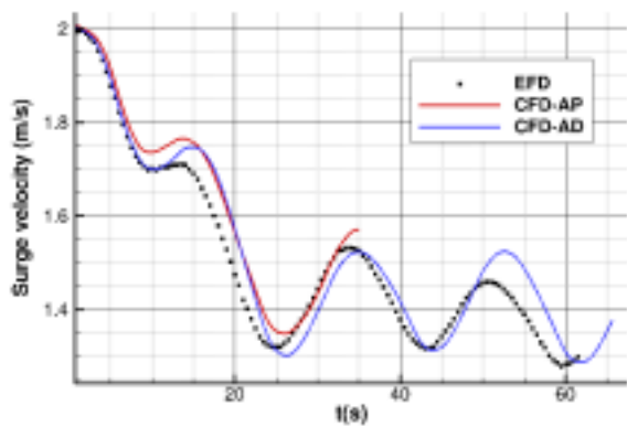
Fig.18 Time history of surge velocity for the KCS zz2020 motion
