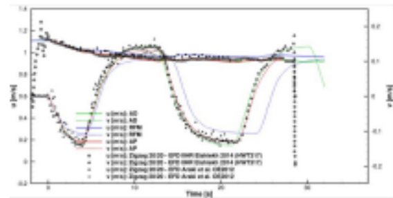
Fig. 8 Time history of the ship speed components (surge u , sway v )
