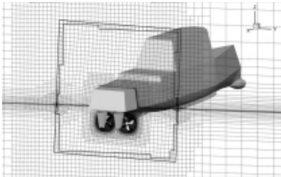
Fig. 3 Adapted grid in longitudinal plane through propeller centers at an arbitrary time instant
