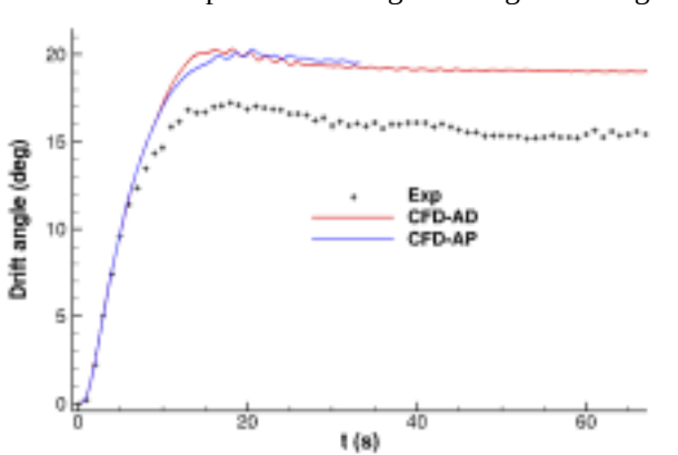
Fig.24 Time history of drift angle for the KCS TC35 motion
