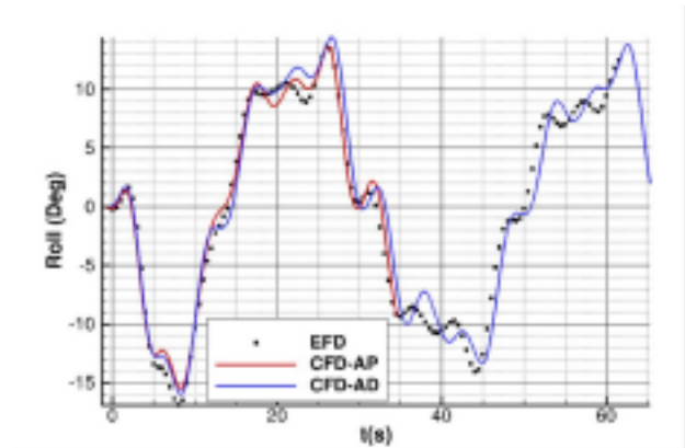
Fig.17 Time history of the roll angle for the KCS zz2020 motion
