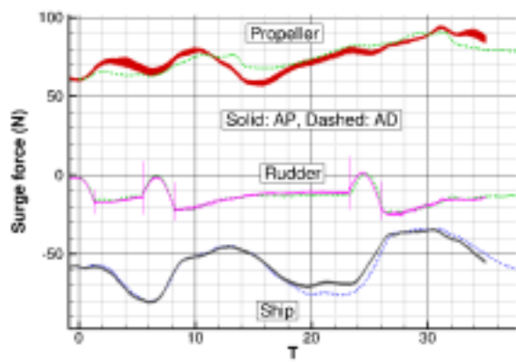
Fig.19 Time history of surge forces for the KCS zz2020 motion
