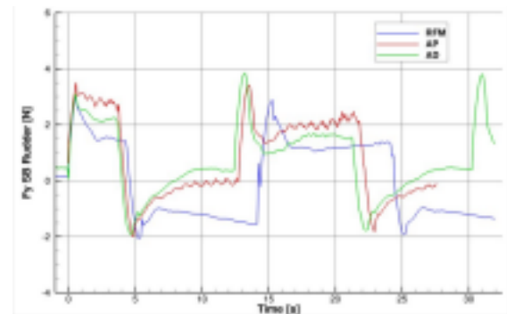
Fig. 9 Time history of transversal force F_y on the starboard rudder (in the frame linked to the rudder)
