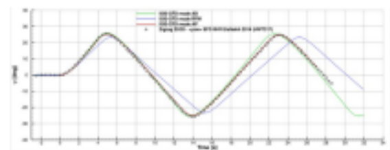
Fig. 10 Time history of the yaw angle
