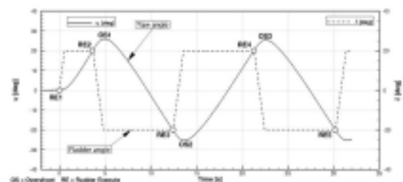
Fig. 5 20^\circ/20^\circ zigzag rules and notations where RE means Rudder Execute, OS for overshoot of the computed ship's yaw \psi and \delta is the controlled rudder angle.
