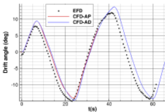
Fig.20 Time history of drift angle for the KCS zz2020 motion
