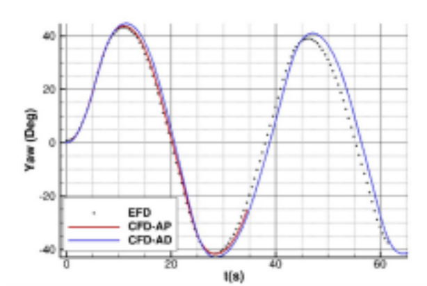
Fig. 15 Time history of yaw angle for the KCS zz2020 motion
