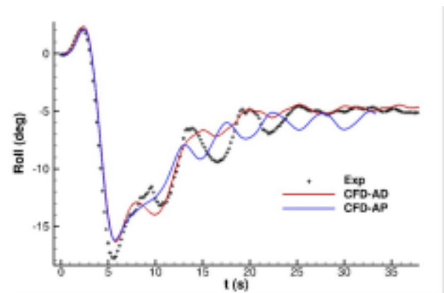
Fig.26 Time history of roll angle for the KCS TC35 motion
