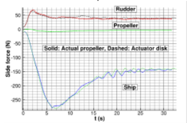
Fig.25 Time history of side force for the KCS TC35 motion
