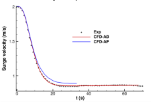
Fig.22 Time history of surge velocity for the KCS TC35 motion
