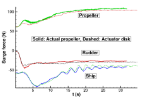
Fig. 23 Time history of surge force for the KCS TC35 motion
