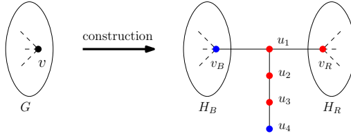
Fig. 3. Reduction from DOMINATING SET to RED-BLUE SEPARATION of Theorem 2.
