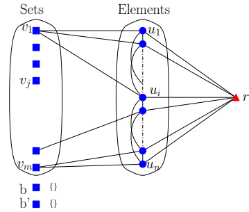
Fig. 2. Reduction from SET COVER to RED-BLUE SEPARATION of Theorem 1.
