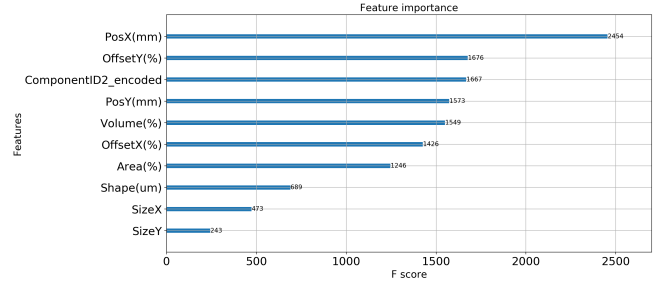
Figure 2. Task 1: feature importance of the XGBoost classifier
