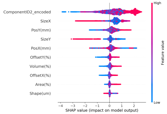
Figure 6. Task 1: SHAP value of the XGBoost classifier
