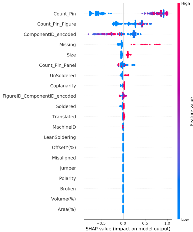
Figure 9. Task 3: SHAP value of the XGBoost classifier
