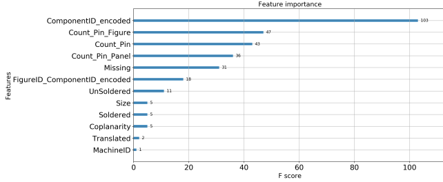
Figure 5. Task 3: feature importance of the XGBoost classifier
