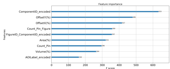
Figure 4. Task 2: feature importance of the XGBoost classifier for the three-tuple (AOI defect is not linked to a pin)
