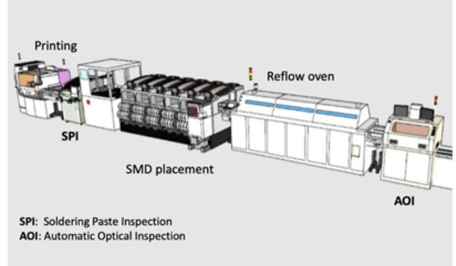
Figure 1. Surface Mount Technologies Production Line. (PHM Society, 2022)
