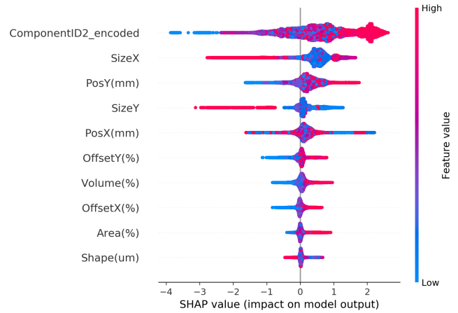
Figure 6. Task 1: SHAP value of the XGBoost classifier
