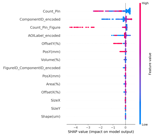
Figure 7. Task 2 for the four-tuple (AOI defect is linked to a pin): SHAP value of the XGBoost classifier
