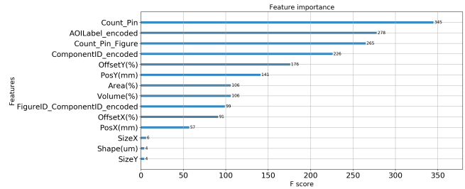
Figure 3. Task 2: feature importance of the XGBoost classifier for the four-tuple (AOI defect is linked to a pin)
