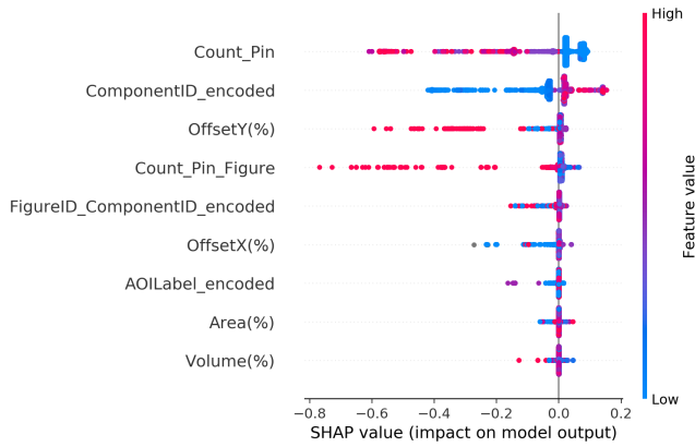
Figure 8. Task 2 for the three-tuple (AOI defect is not linked to a pin): SHAP value of the XGBoost classifier
