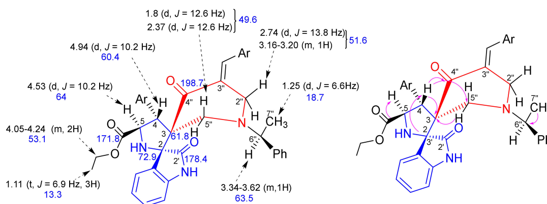
Figure 3. ^1\text{H} (black) and ^{13}\text{C} NMR (blue) chemical shifts along with selected HMBC correlations of 4c .
