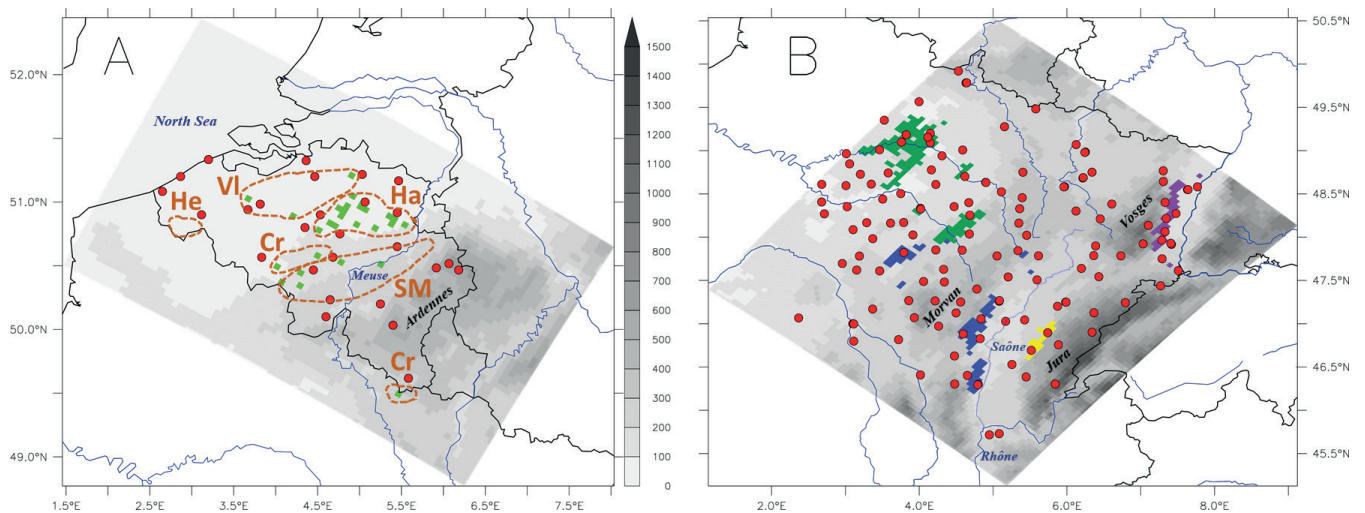
FIGURE 1. Model topography (greyscale in metres), location of the weather stations (red dots) used in this study and viticultural regions (in coloured pixels; light green: Belgium Wine Region (BWR), dark green: Champagne, blue: Bourgogne, yellow: Jura, purple: Alsace) on the domain covering Belgium (A) and on the domain covering the northeast quarter of France (B). The Protected Designation of Origin (PDO) or Geographical Indications (GI) of each BWR pixel is identified with dashed orange lines on map A with acronyms. He=Heuvelland; Ha = Hageland and Haspengouw; VI = Vlaamse landwijn; SM = Côtes de Sambre et Meuse; Cr = Crémant de Wallonie (i.e., sparkling wine). Toponyms related to rivers and sea are in blue letters. Toponyms relative to the reliefs are in black letters.
