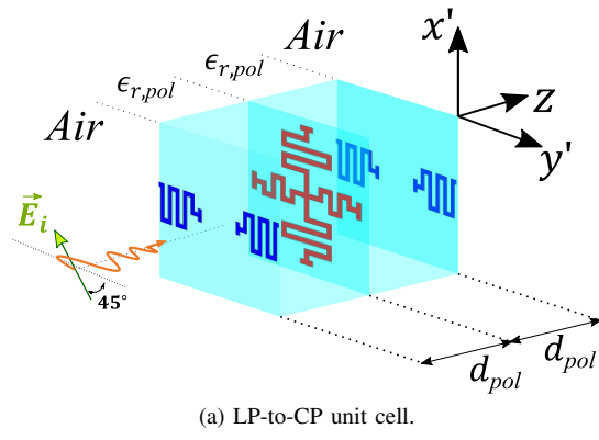
(a) LP-to-CP unit cell.
