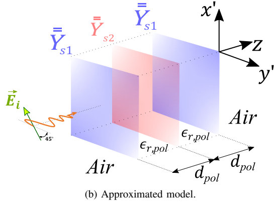
Fig. 14: (a) Unit cell of the LP-to-CP converter. (b) Equivalent model based on admittance boundary conditions. Simulations are carried out in periodic environment considering d_{pol} = 1.524 mm, \epsilon_{r,pol} = 3 , and \mathbf{E}_i = E_{i,x}\hat{x} .
