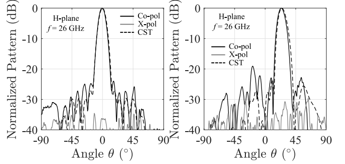
(b) Horn #1.
