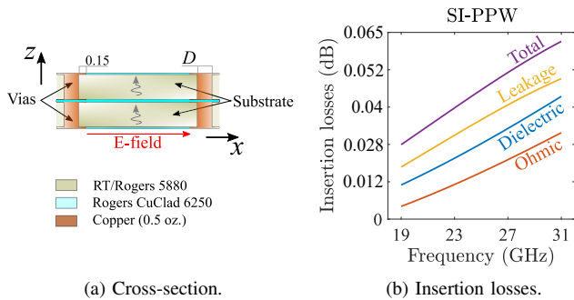
Fig. 3: (a) Cross-section of the SI-PPW in the xz -plane. (b) Simulated insertion losses for the SI-PPW. The via diameter is D = 3 mm. All other dimensions are given in millimeters.
