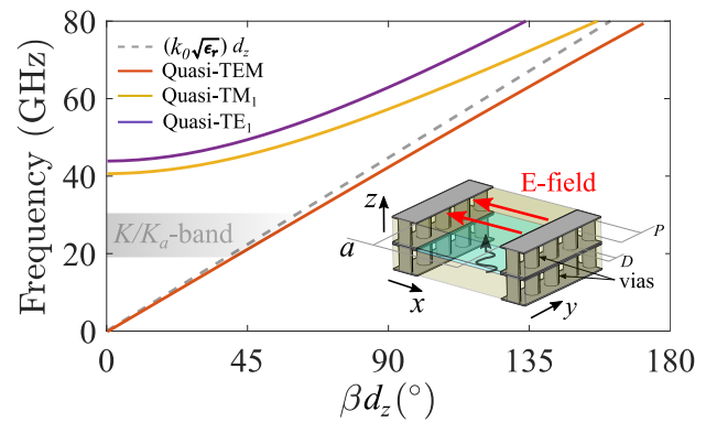
Fig. 2: Dispersion diagram of the SI-PPW. Geometrical parameters: D = 0.3 mm, P = 0.6 mm, a = 2.13 mm, \epsilon_r = 2.2 , and d_z = 1.1 mm.
