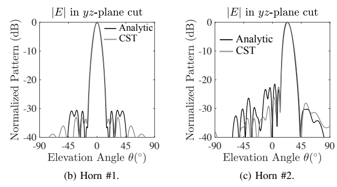
Fig. 10: (a) Simulated input reflection coefficients. (b)-(c) Simulated radiation patterns at 25 GHz of the antenna for horn #1 and #2 excitations, respectively.
