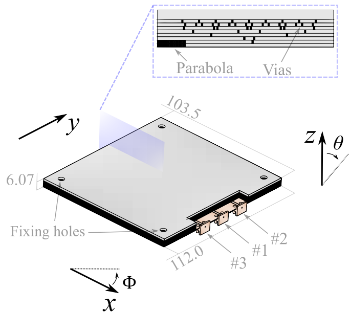
Fig. 1: Perspective view of the antenna architecture with the stack-up shown. Dimensions are given in millimeters.
