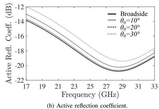
Fig. 4: (a) Simulation setup of the radiating cell of the CTS array in PCB technology. (b) Simulated active reflection coefficient of the array's unit cell. The results are shown for four beam directions along the yz -plane (H-plane). Geometrical parameters: a = 2.13 mm, d = 2.73 mm, l = 1.544 mm, d_z = 0.508 mm, D = 0.3 mm, P = 0.6 mm, and \epsilon_r = 2.2 .
