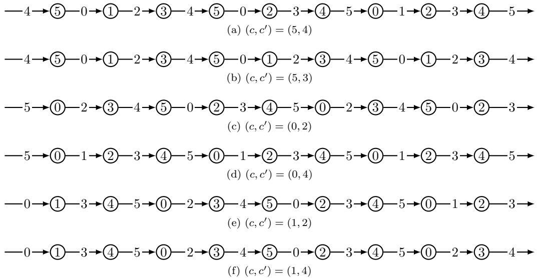
Figure 8: \vec{T} -total-colorings \tau of \vec{P} , showing that Lemma 5.9 is true.
