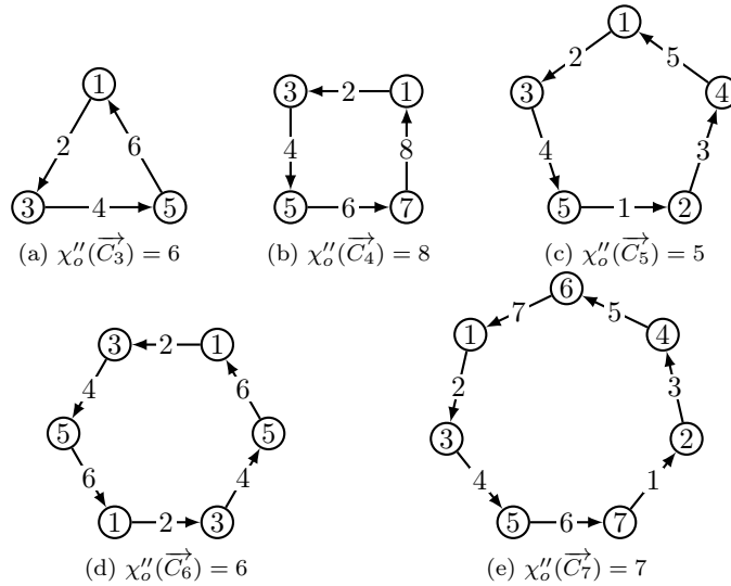
Figure 3: The unique optimal oriented total-colorings of small directed cycles.
