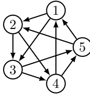
Figure 2: The tournament \vec{T}_5 .
