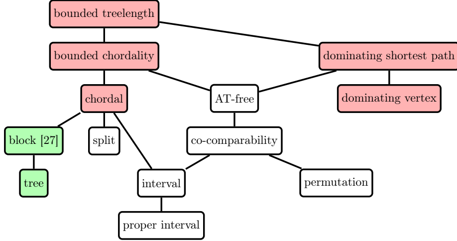
Figure 1: Inclusion diagram for graph classes discussed here (and related ones). If a class A has an upward path to class B , then A is included in B . For graphs in the green classes, ISOMETRIC PATH COVER is polynomial-time solvable; for graphs in the red classes, it is NP-complete. The white classes are still open. For all shown graph classes, ISOMETRIC PATH COVER is constant-factor approximable in polynomial time.
