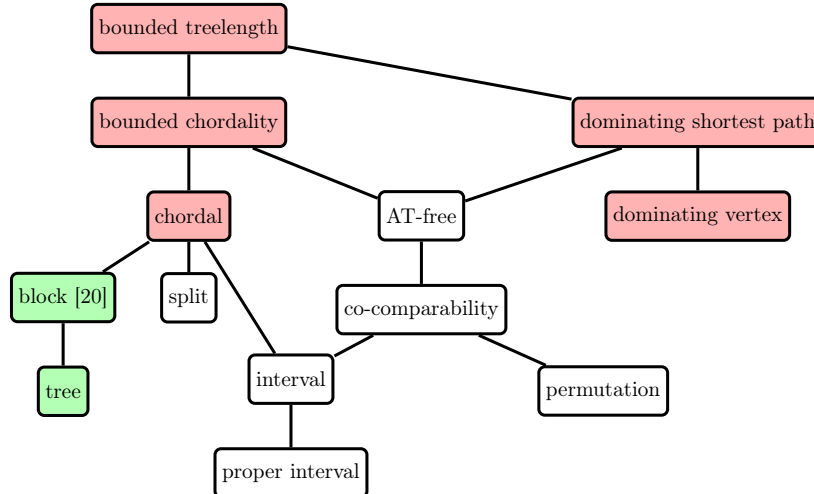
Figure 1: Inclusion diagram for graph classes discussed here (and related ones). If a class A has an upward path to class B , then A is included in B . For graphs in the green classes, ISOMETRIC PATH COVER is polynomial-time solvable; for graphs in the red classes, it is NP-complete. For all shown graph classes, ISOMETRIC PATH COVER is constant-factor approximable in polynomial time.
