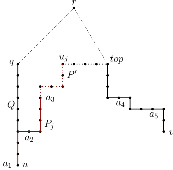
Figure 2: Proof of Claim 25.1. Path P' is dotted, and path P_j is red.
