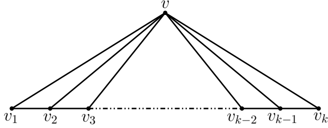
Figure 4: A tight-approximation example for interval graphs
