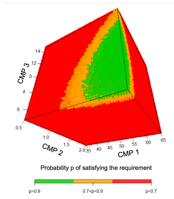
Figure 3: Example of Method Operating Design Region for three method parameters (CMP1 to CMP3). OOS (red); PAR (orange); NOR (green)) are the three constitutive regions defined in Section 3.1. To compensate random variations and drifts of the analytical method, a correction action shall be performed on Critical Method Parameters to keep the operating point in the NOR region
