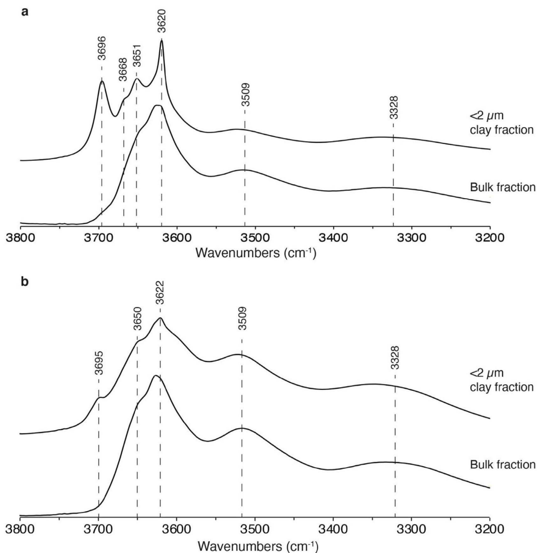
Figure 7. Typical FTIR spectra of kaolin- and sudoite-bearing samples (bulk and <2 \mu\text{m} clay fractions) from the \text{FB}_{2a} unit. The interval from 3800 to 3200 \text{ cm}^{-1} characterizes the hydroxyl-stretching band region. (a) Mat-related structures. (b) Sandstones.
