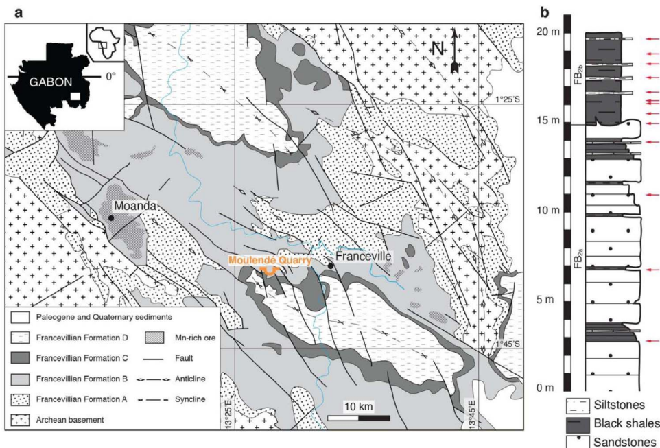
Figure 1. (a) Geological map of the Paleoproterozoic Franceville sub-basin showing the study area—Moulend  Quarry [modified from Bouton et al. , 2009]. (b) Lithostratigraphic column of the FB 2 Member in the Moulend  Quarry displaying sampling positions of both microbial mat structures and host sediments (red arrows). Images in (a) and (b) are modified from Aubineau et al. [2020] and Aubineau et al. [2019], respectively.
