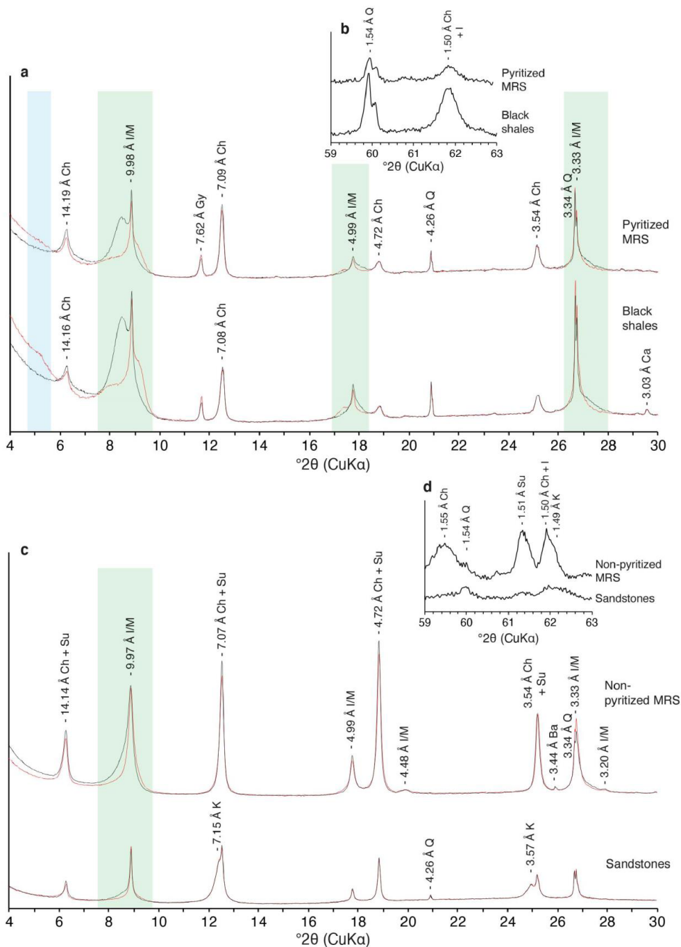
Figure 4. Representative XRD patterns of the <2 \mu\text{m} clay fraction of mat-related structures and host sediments in the FB 2b Member (a, b) and FB 2a Member (c, d). (a, c) Oriented preparations after air-drying (black lines) and glycolation (red lines). (b, d) XRD profiles of 060 reflection of randomly oriented preparations. The blue and green areas correspond to R0 I-S MLMs and R3 I-S MLMs, respectively, as previously described in Aubineau et al. [2019]; chlorite (Ch); illite/mica (I/M); gypsum (Gy); quartz (Q); calcite (Ca); sudoite (Su); barite (Ba); kaolinite (K).
