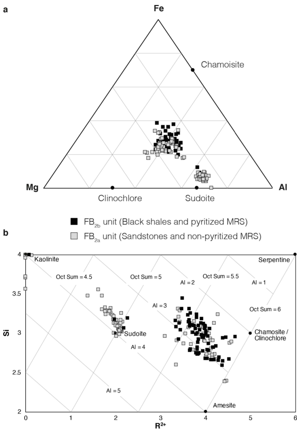
Figure 6. Projection of the structural formulas of chlorite minerals from the FB_2 Member. (a) EDX analyses of chlorite plotted in the triangular diagram Mg–Fe– Al_T [Velde, 1985]. (b) Chemical compositions of chlorite projected on the Si versus R^{2+} diagram, as designed by Wiewióra and Weiss [1990]. Data are expressed in atoms per half unit cell. The octahedral occupancy and total number of Al atoms per half unit cell are shown by contours.
