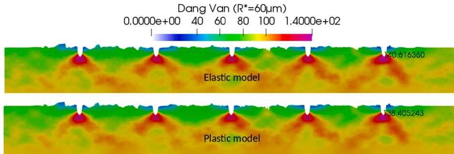
Fig. 18. Distribution of the Dang Van stress ( R^* = 60 \mu\text{m} ) in defective polycrystalline aggregates using plastic and elastic constitutive models respectively with realistic texture after a cyclic tension loading at 150 MPa.
