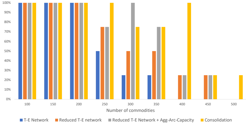
(a) Percentage of instances solved
