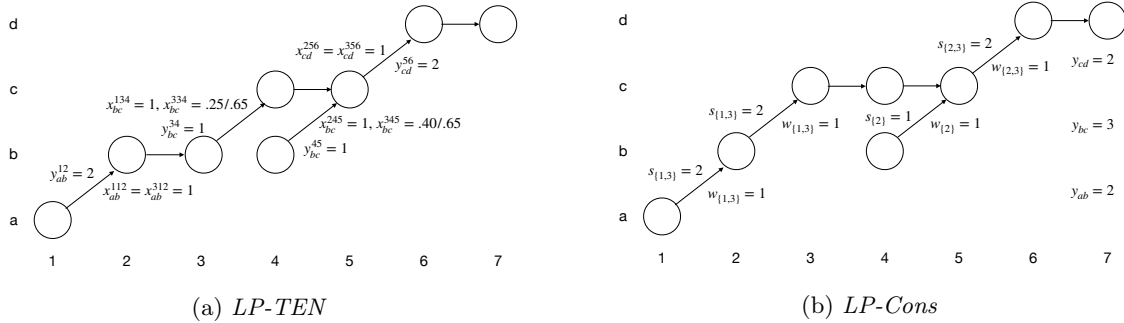
Figure 2: Optimal linear programming solutions for example in Figure 1 and Table 1.
