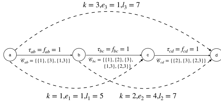
Figure 1: Network \mathcal{N} and commodities \mathcal{K} in example
