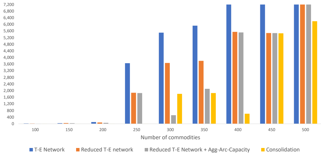
(b) Average time to termination (seconds)
