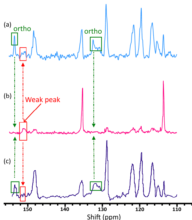
Fig. 7. A comparison of the experimental ^{13}\text{C} -NMR spectra for (a) the commercial OAPS, (b) the controlled OAPS and (c) the OAPS prepared by Krishnan et al. [86], all of them in \text{DMSO-d}_6 , along with a proposed assignment for ortho -specific peaks.
