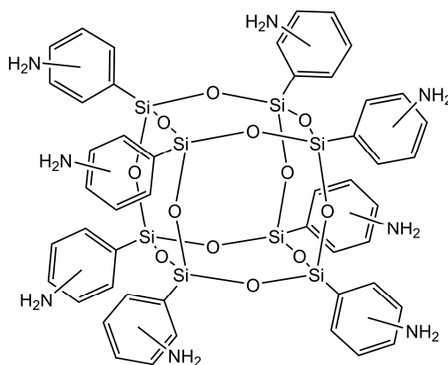
Fig. 1. The general structure of octa(aminophenyl)silsesquioxane (OAPS) [5, 6] The \text{NH}_2 group on each phenyl ring can either be in the meta , ortho or para position.
