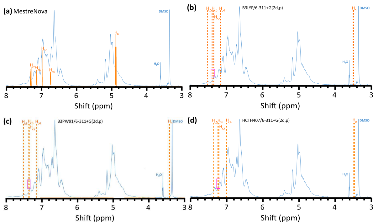
Fig. 12. A comparison of the commercial OAPS ^1\text{H} -NMR experimental spectrum (blue line) with the chemical shifts predicted for the aromatic and amine hydrogens of meta -OAPS by (a) MestreNova (lines) and (b-d) Gaussian (dashed lines) using different DFT functionals along with the 6-311+G(2d,p) basis set.
