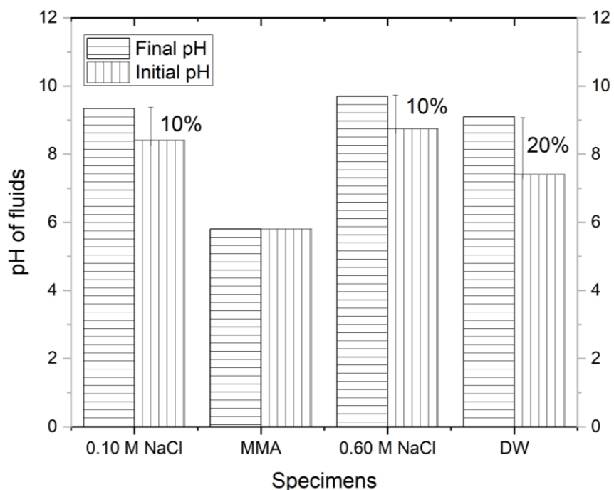
213 Fig. 4 Final pH measured in the effluents and compared with the initial pH of the respective fluids at the end of 5 W-D cycles.
