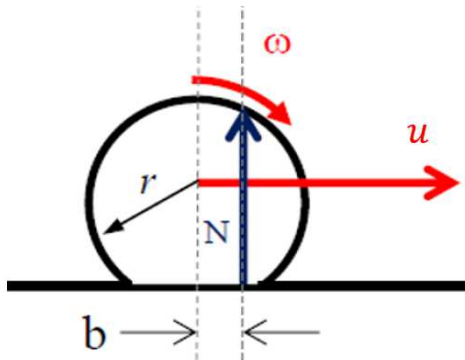
Figure 2 : Rolling resistance model
