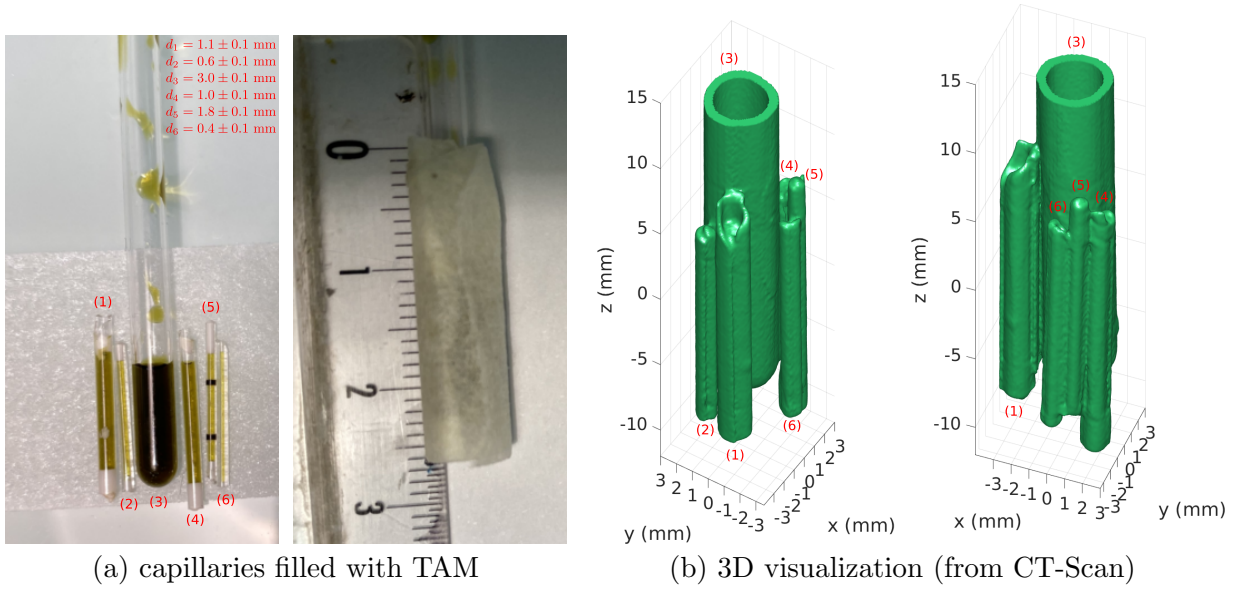
Figure 16: Capillary tubes filled with TAM. We filled six tubes with a solution of TAM with concentration 1 mM. The tubes, numbered from one to six, and their internal diameters ( d_i ) _{1 \leq i \leq 6} , are visible in (a) (left). The tubes were wrapped together using masking tape, as displayed in (a) (right). We performed a CT-Scan acquisition of the sample, leading to the reconstruction of a 3D image of the wrapped tubes. An isosurface of the 3D image is displayed in (b) under two different orientations, showing the tubes organization inside the masking tape (the latter being transparent to X-rays). Some slices of the 3D image are also displayed in Figure 17, where we can visualize the TAM solution contained inside the tubes.
