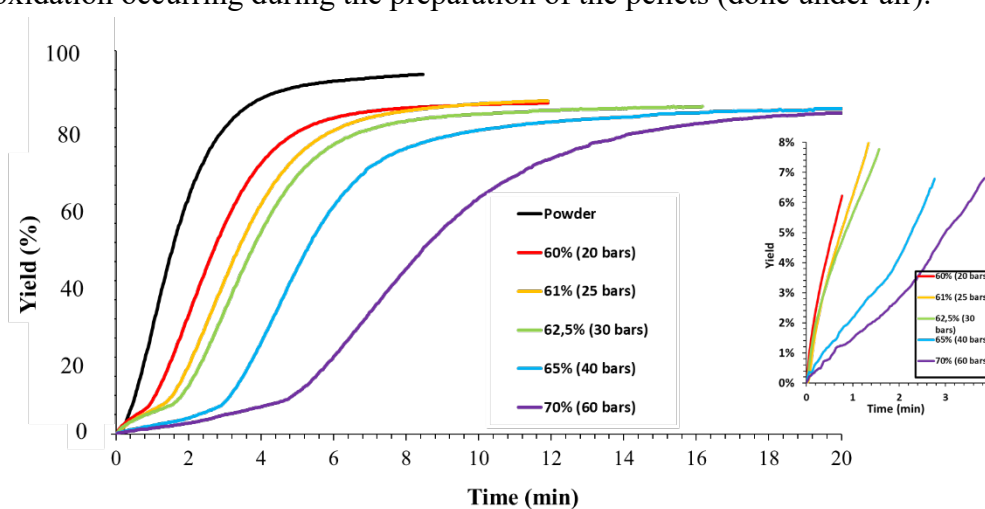
Figure 4 : Yield of H_2 produced as a function of the compactness ( i.e. the applied pressure to fabricate the pellets) of AZ33-5wt.%C pellets. The inset highlights the influence of the compacity on the initial “straight” slope and duration of incubation time (discussed in figure 5).
