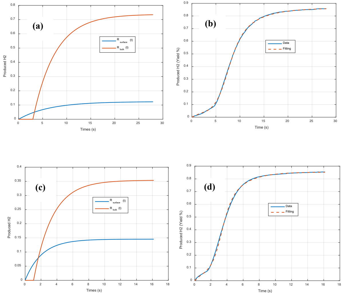
Figure 7: (a and c) representation of the two functions separately to illustrate the temporal placement (for the pellet with 70 % and 62.5 % compactness), (b and d) fitting of the hydrolysis yield for the mixtures AZ33 + 5% C ball milled for 3 h and compressed at 70% and at 62,5%, respectively .
