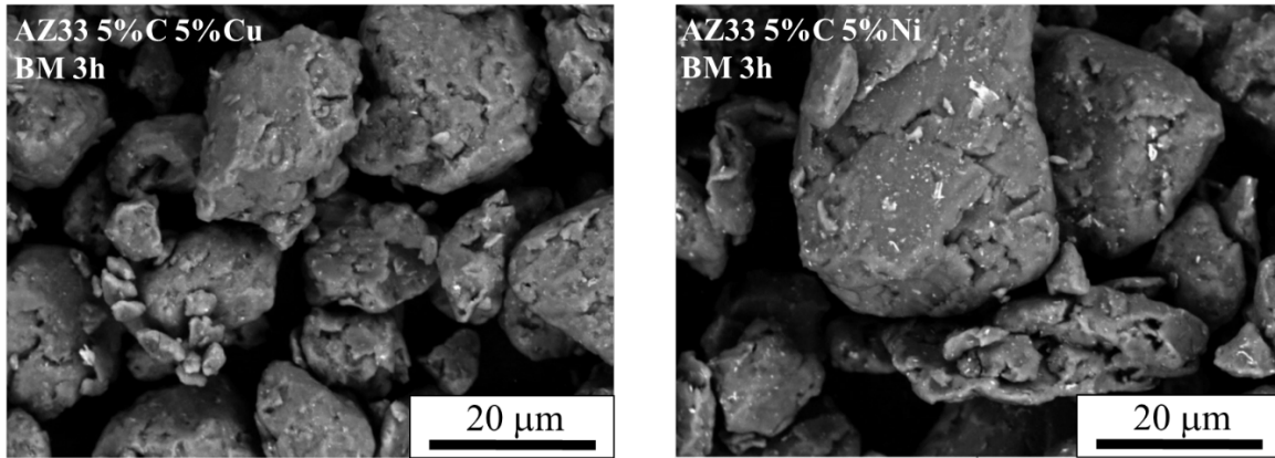
Figure 2 : SEM micrographies obtained after 3h of ball milling for the mixtures AZ33 +5wt.%C + 5wt.%Cu (left) and AZ33 + 5wt.%C + 5wt.%Ni (right) using backscattered electrons.
