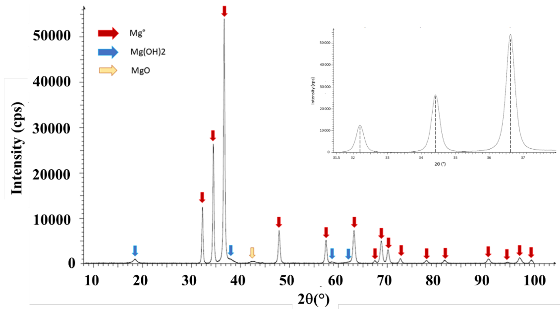
Figure 1 : XRD patterns of the initial powdered material
