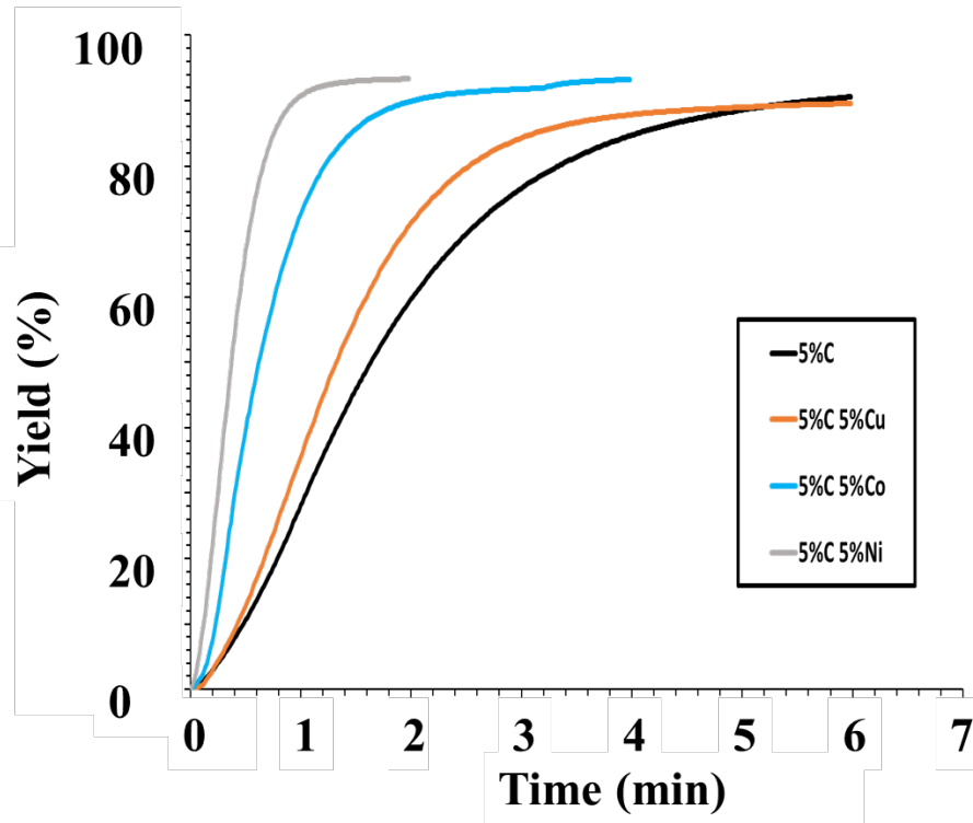
Figure 3: Yield of H_2 produced as a function of time during the hydrolysis reaction of different mixtures ball milled for 3h.
