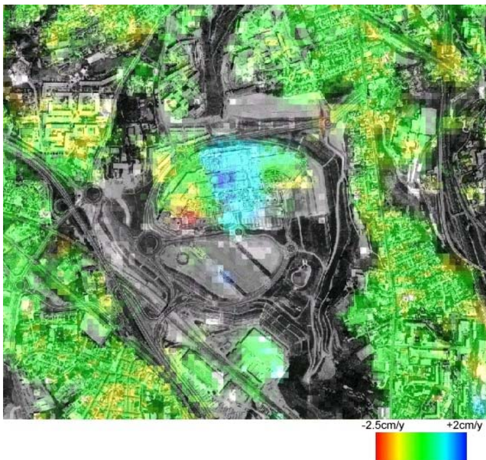
Fig. 4. Map of the mean displacement rate between 1997 and 2000 around the “Grand littoral” centre
