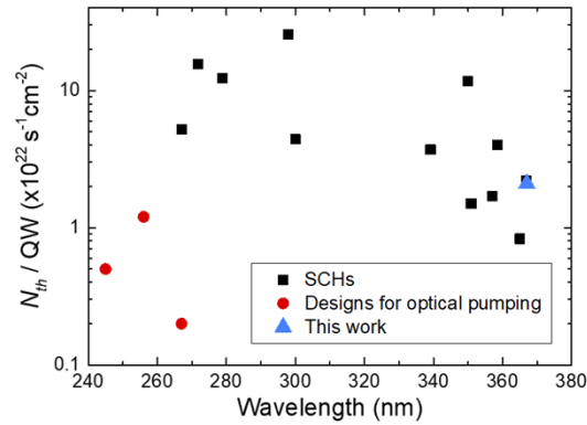
Fig. 10. Variation of N_{th} per QW as a function of the emission wavelength (data from Table 1). Data corresponding to SCHs and heterostructures optimized for optical pumping are represented with different symbols and colors.
