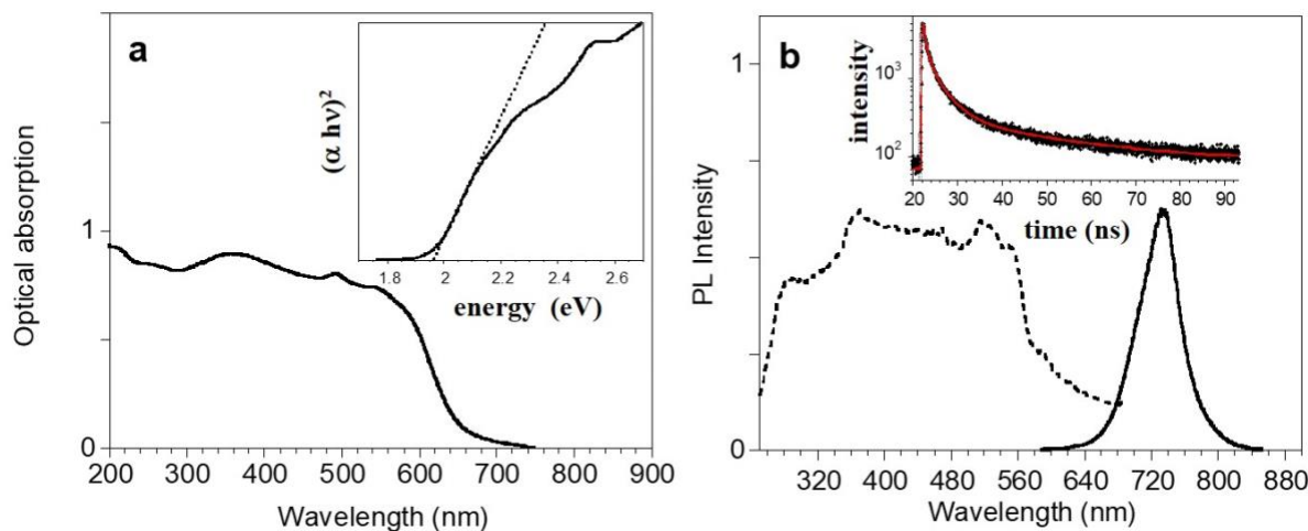
Figure 3. a) Optical absorption, Tauc Plot (inset) b) PL (solid line) and PLE spectra (dashed line) of (\text{FA})_3(\text{HEA})_2\text{Pb}_3\text{I}_{11} . Excitation wavelength 540nm, emission 740nm. In the inset the emission decay (solid points) recorded at 740nm with three-exponential fit (red solid line) are reported. Fitting parameters: (0.2845) 3.707ns; (0.6694) 0.803ns; (0.0460) 29.76ns; \chi^2=1.31081 .
