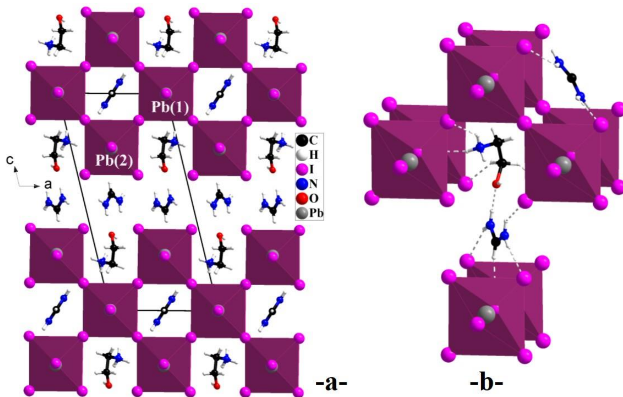
Figure 1. Structure of the \langle 1\ 1\ 0 \rangle -oriented hybrid perovskite (FA) 3 (HEA) 2 Pb 3 I 11 : General view along the b direction (a) and partial view showing FA + cations localized both in the inner cavity of the perovskite sheet and in the interlayer space and HEA + cations localized in outer perovskite cavities (b) (dashed lines: H...I and H...O contacts < 3.10 Å).
