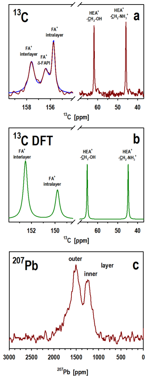
Figure 2. a) Direct excitation ^{13}\text{C} spectrum of (\text{FA})_3(\text{HEA})_2\text{Pb}_3\text{I}_{11} (red) and deconvolution of the \text{FA}^+ signal group with three lorentzians (blue). b) Simulated ^{13}\text{C} spectrum based on the chemical shieldings extracted from a DFT calculated electronic structure. c) ^{207}\text{Pb} spectrum.
