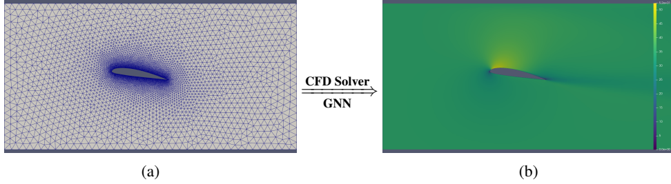
Figure 1: (a) Airfoil mesh. (b) x -velocity field. The goal of a GNN is to produce outputs that are as accurate as those of a CFD solver while drastically reducing the computational time.
