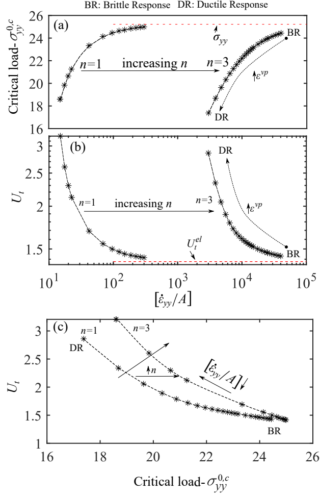
Fig. 11. Critical load (a) and energy density until failure (b) as function of the ratio [\dot{\epsilon}_{yy}/A] . The critical load ( \sigma_{yy}^{el,0,c} ) and the energy density until failure ( U_t^{el} ) in the case of an elastic brittle material are also shown. The direction of the increase in viscoplastic strain ( \epsilon^{vp} ) at the crack tip is illustrated. (c) Correlation between the critical load and the energy density until failure. For all simulations, the initial crack length was set to a_0 = l_c .
