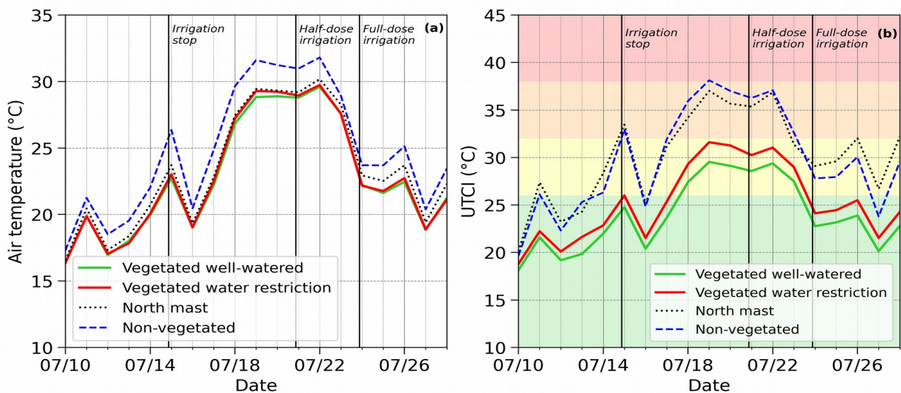
Figure 5. a) Evolution of the air temperature averaged from 11h to 13h UTC at 0.4 m from the ground, b) evolution of the UTCI averaged from 11h to 13h UTC at 0.4 m from the ground regarding the different thermal stress categories: no thermal stress (9 to 26 °C UTCI, green), moderate heat stress (26 to 32 °C UTCI, yellow), high heat stress (32 to 38 °C UTCI, orange), very high heat stress (38 to 46 °C UTCI, red) and extreme heat stress (>46 °C UTCI, not shown).
