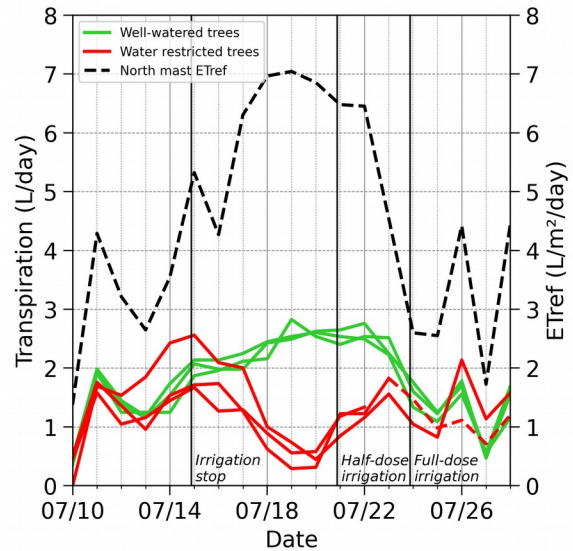
Figure 3. Evolution of the daily transpiration estimated for the 3 central trees of each zone and the corresponding local reference evapotranspiration E_{Tref} . Red dotted line: only 1 ECH20 EC-5 working, red solid line stopped on July 22: no more ECH20 EC-5 working.
