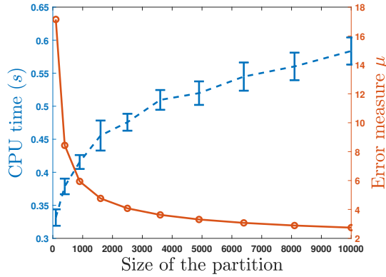
Fig. 8. Line in blue represents the average time of execution with respect to the number of cells in the partitions, with bars representing the standard deviation. Line in orange represents the performance criterion \mu(\mathcal{D}, \mathcal{Q}) with respect to the number of cells in the partitions.
