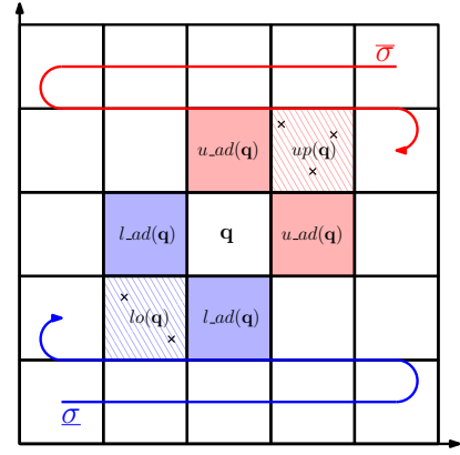
Fig. 5. A representation of the sets \text{up}(\mathbf{q}) , \text{u\_ad}(\mathbf{q}) , \text{lo}(\mathbf{q}) , \text{l\_ad}(\mathbf{q}) and the order in which we calculate \overline{\sigma} and \underline{\sigma} .
