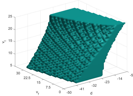
Fig. 9. Controllable set of the symbolic controller enforcing the assume-guarantee contract (39) for system (38)
