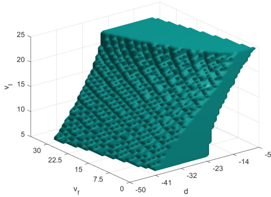
Fig. 9. Controllable set of the symbolic controller enforcing the assume-guarantee contract (39) for system (38)
