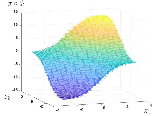
Fig. 6. Map F(\mathbf{z}) with w = 0 everywhere is represented in solid. The upper and lower bounds of the over-approximation are represented in transparency
