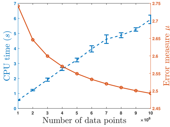
Fig. 7. Line in blue represents the average time of execution with respect to the number of data points, with bars representing the standard deviation. Line in orange shows the relation between the number of points and the performance criterion \mu(\mathcal{D}, \mathcal{Q}) .
