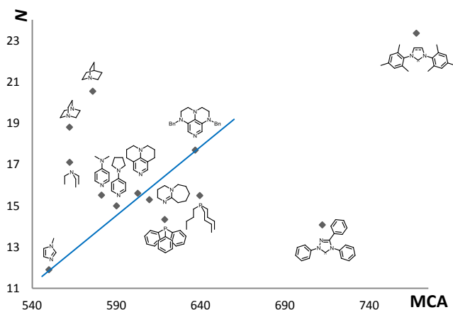
Figure 7. Nucleophilicity N against Lewis basicity MCA, for a selection of organocatalysts.
