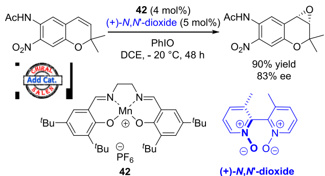
Scheme 53. Asymmetric epoxidation with achiral (salen)Mn complex 42 catalyzed and an enantiopure additive
