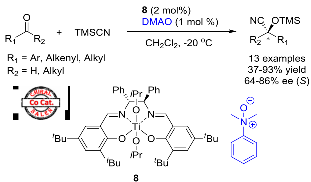
Scheme 12. Catalytic enantioselective cyanosilylation of ketones developed by Feng et al.
