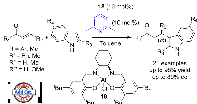
Scheme 49. Stereoselective addition of indoles to ( E )-enones catalysed complex 18 with 2,6-lutidine
