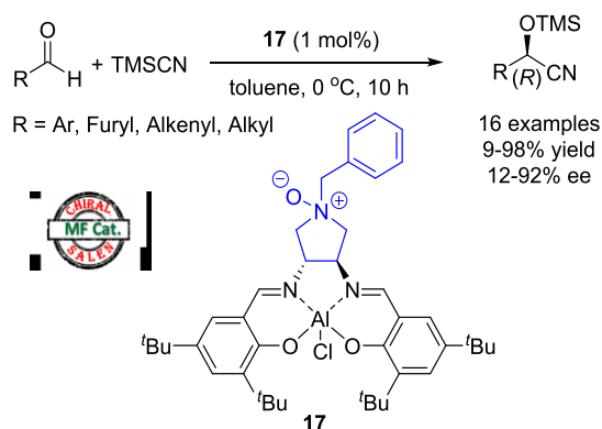
Scheme 19. Enantioselective cyanosilylation of aldehydes catalysed by Al salen bifunctional catalyst 17
