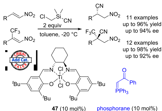
Scheme 62. hydrocyanation of nitroalkenes with 47 and phosphorane additive
