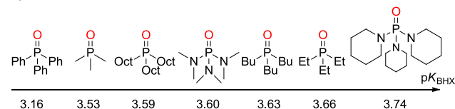
Figure 9. Hydrogen-bond affinity (p K BHX ) for a range of phosphane oxides.
