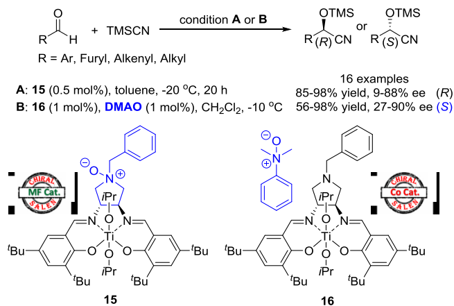
Scheme 18. Catalytic enantioselective cyanosilylation with the ‘two-center catalyst’ developed by Sun’s group
