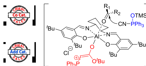
Scheme 25. Cyanosilylation catalyzed by (salen)AlCl 18 , TPPO and phosphorane as co-catalysts
