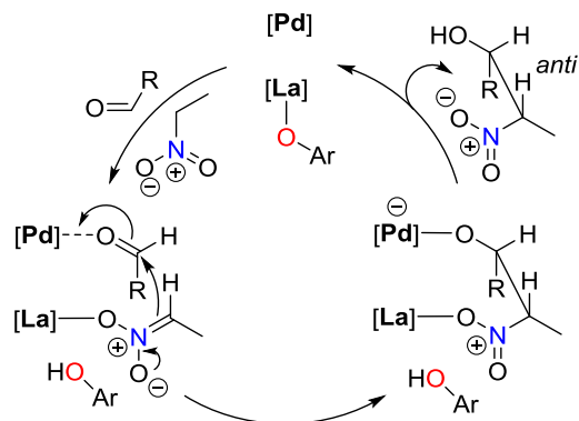
Scheme 71. Mechanism of Henry reaction with trifunctional catalyst 57
