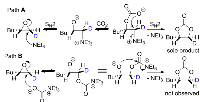
Scheme 36. (salen)Cr III / N -methylimidazole catalyzed copolymerization of epoxide with CO 2
