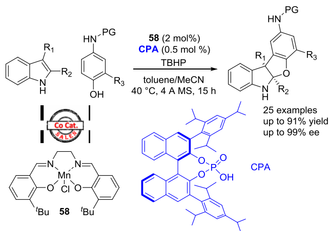
Scheme 72. Enantioselective indole/aminophenol oxidative [3+2] cycloaddition catalysed by achiral 58 and CPA
