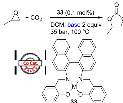
Scheme 37. Carbonate formation from propylene oxide catalyzed by rac -Binam salen complex 33 and nitrogen bases
