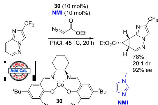
Scheme 48. Enantioselective cyclopropanation by (salen)Co complex 30 and NMI as co-catalyst
