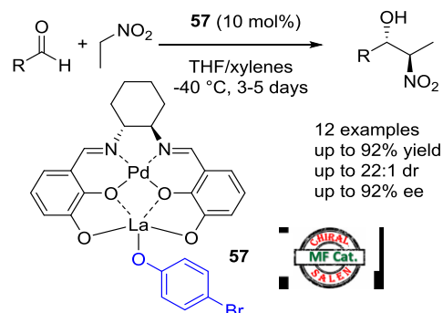
Scheme 70. Asymmetric Henry reaction catalyzed catechol-salen Pd/La complex and 4-bromophenol
