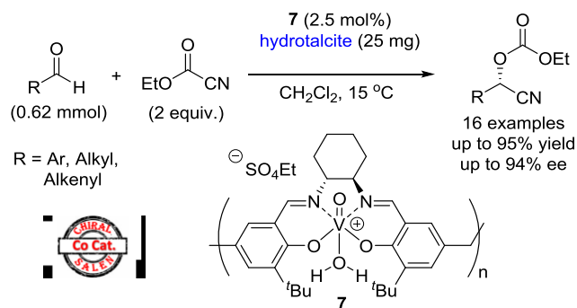
Scheme 10. Enantioselective addition of ethyl cyanofornate to various aldehydes using a polymeric (salen) V complex together with hydrotalcite
