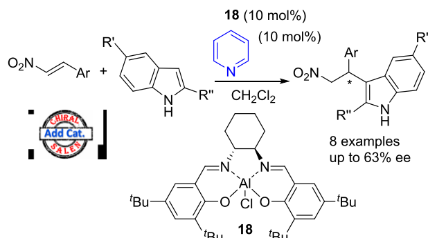
Scheme 50. Stereoselective alkylation of indoles with nitroalkenes catalysed by complex 18 with pyridine
