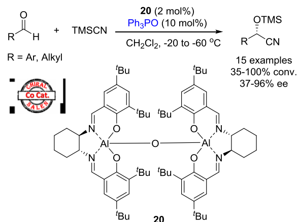
Scheme 23. Cyanosilylation of aldehydes with bimetallic catalyst 20 and TPPO as co-catalyst
