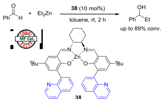
Scheme 44. Addition of diethylzinc to aldehydes using (salen)Zn complex 38 containing a quinoline base (chiral induction was not reported)
