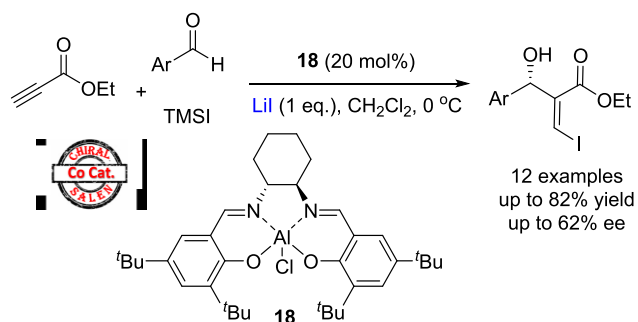
Scheme 59. Asymmetric catalytic synthesis of \beta -halo MBH ester adducts catalysed by complex 18
