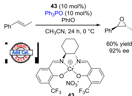
Scheme 56. ( E )-alkene epoxidation with cationic complex 43 and TPPO
