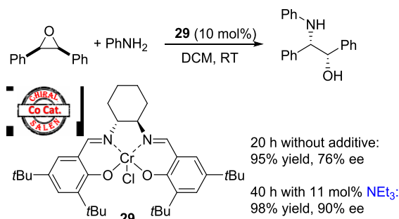
Scheme 33. Anilinolysis of epoxides catalysed by complex 29
