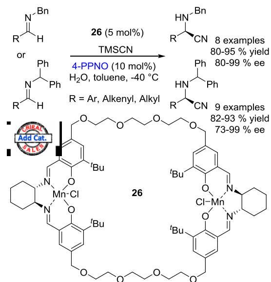
Scheme 30. Asymmetric Strecker reaction of benzyl- and benzhydrylimines with TMSCN catalysed by 26 and 4-PPNO as co-catalyst
