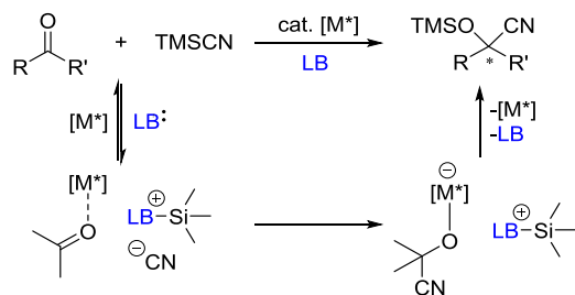
Scheme 11. General mechanism of cyanosilylation under co-catalysis
