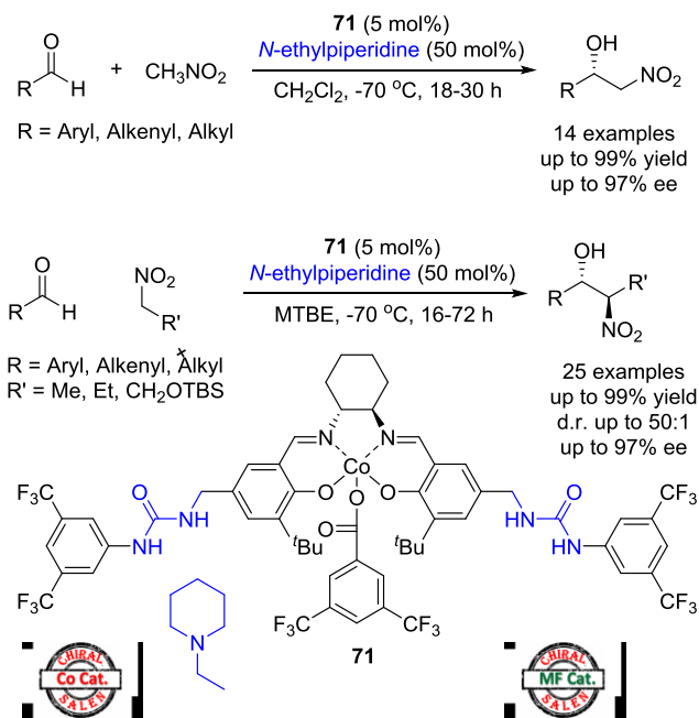
Scheme 87. Henry reactions with (salen)Co-OBz F bisurea catalyst 71
