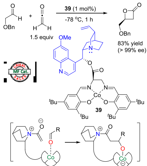
Scheme 46. Cycloaddition of aldehydes and ketene catalyzed by complex 39
