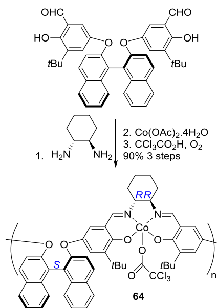
Scheme 77. Synthesis of chiral polymeric (BINOL-salen)Co catalyst 64
