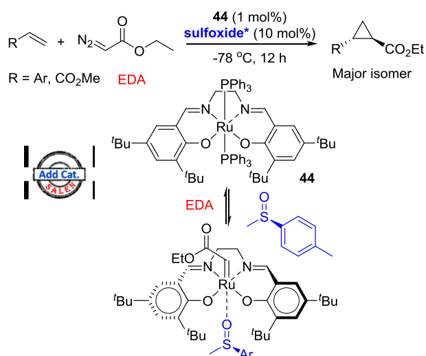
Scheme 57. Olefins cyclopropanation with achiral Ru II complex 44 using chiral sulfoxides
