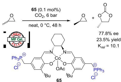
Scheme 78. Synthesis of chiral carbonates with complex 65 bearing an appended phosphonium salt
