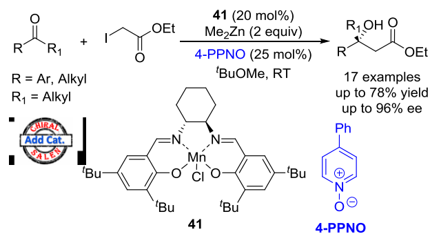
Scheme 54. Catalytic enantioselective Reformatsky reactions promoted by 41 and 4-phenylpyridine N -oxide
