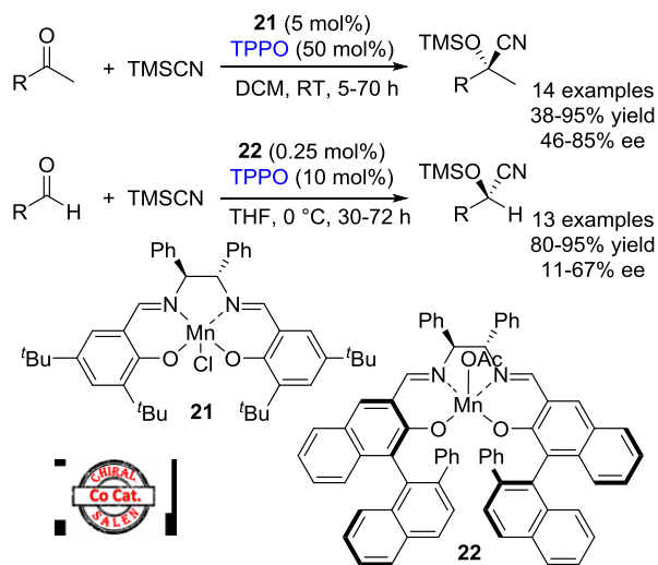
Scheme 26. Enantioselective cyanosilylation of ketones and aldehydes with (salen)Mn III catalysts
