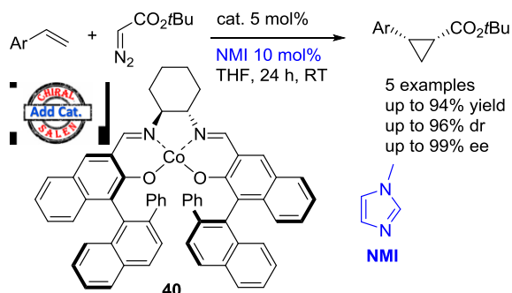
Scheme 47. Enantioselective cyclopropanation of styrenes
