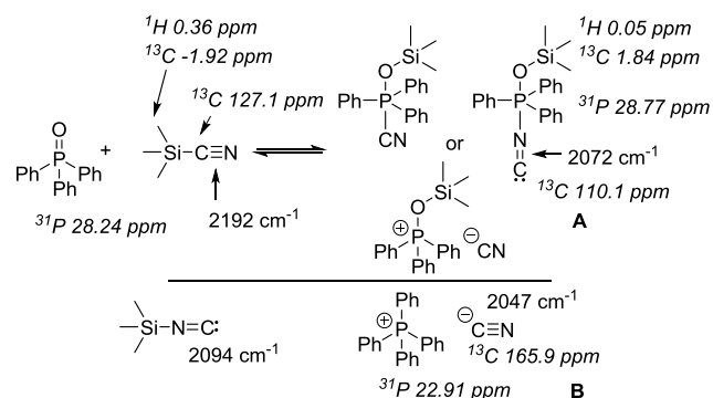
Scheme 21. Potential structures resulting from nucleophilic attack of TMSCN by TPPO (IR in cm -1 and 1 H NMR in ppm)
