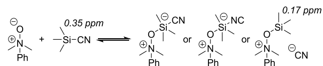
Scheme 13. Potential structures resulting from nucleophilic attack of TMSCN with DMAO
