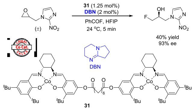
Scheme 35. Synthesis of fluoromisonidazole using dimeric catalyst ( R,R,R,R )- 31 and DBN
