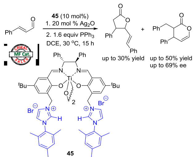
Scheme 58. Synthesis of enol- \delta -lactones by cooperative NHC/(salen)Ti/Ag catalysis with precatalyst 45
