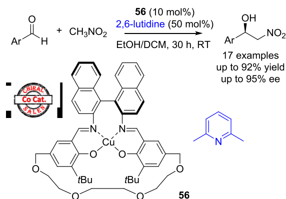
Scheme 69. Asymmetric Henry reaction catalyzed by 56 and 2,6-lutidine
