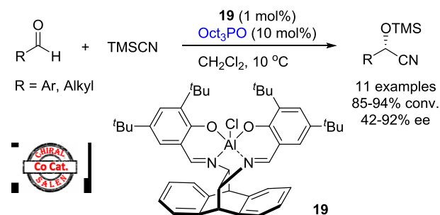
Scheme 22. (Salen)AlCl catalyst 19 based on an anthracene-derived diamine
