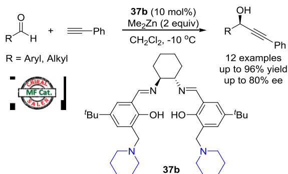
Scheme 45. Asymmetric addition of phenylacetylene to aldehydes catalyzed by in situ generated (salen)Zn complex from ligand 37b
