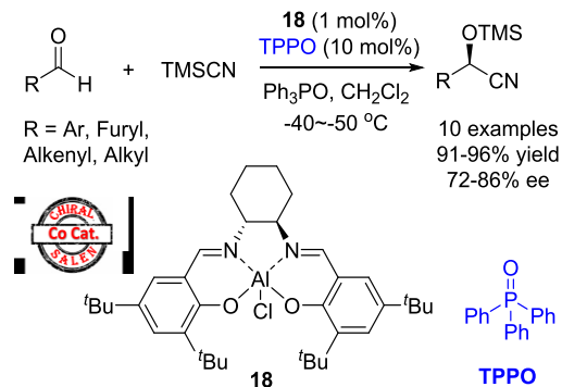
Scheme 20. First example of (salen)AlCl catalysed enantioselective cyanosilylation of aldehydes with TPPO as co-catalyst
