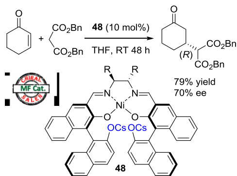
Scheme 63. Bifunctional Ni salen naphthoxide catalyst in the enantioselective Michael addition reaction
