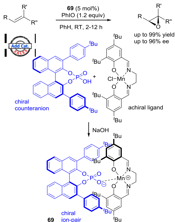
Scheme 84. (Salen)Mn III /chiral phosphate ion pair for catalytic asymmetric epoxidations of unfunctionalized olefins
