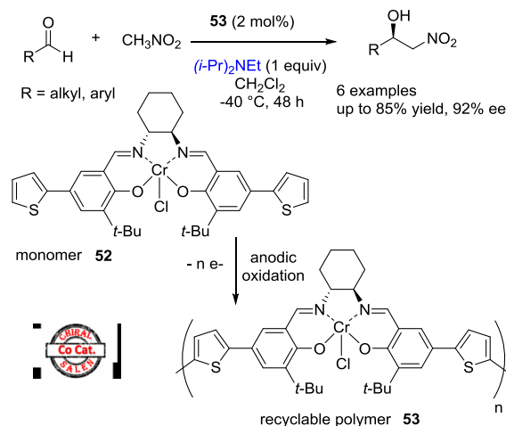
Scheme 67. Chiral thiophene (salen)Cr catalysts 52 and 53 developed by Schulz and co-workers
