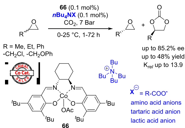
Scheme 79. Asymmetric cycloaddition reaction of CO 2 and epoxides with 66 and chiral ionic liquids
