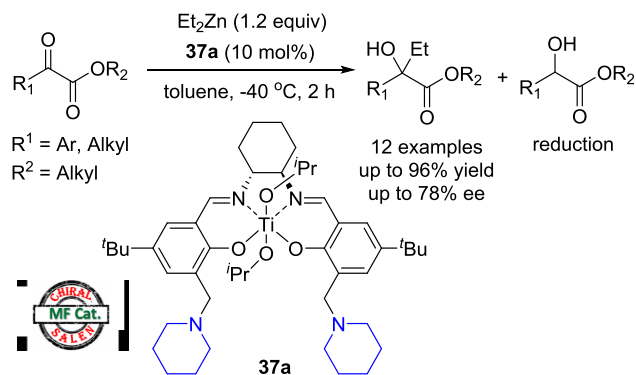
Scheme 43. Addition of diethylzinc to ketoesters using complex 37a containing appended piperidine
