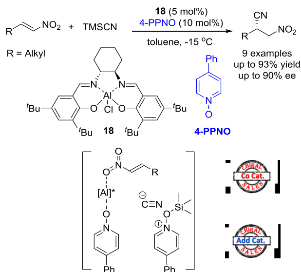
Scheme 55. Asymmetric hydrocyanation of nitroolefins catalyzed by complex 18 and 4-PPNO
