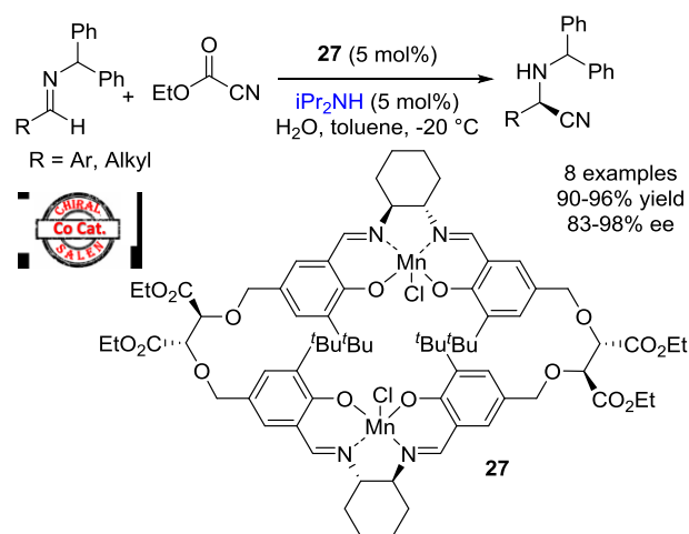
Scheme 31. Asymmetric Strecker reaction with benzhydrylimines and ethyl cyanofornate catalysed by complex 27
