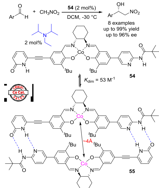
Scheme 68. Self-assembled (Salen)Co 55 , catalyzing asymmetric Henry reaction in presence of DIPEA as co-catalyst
