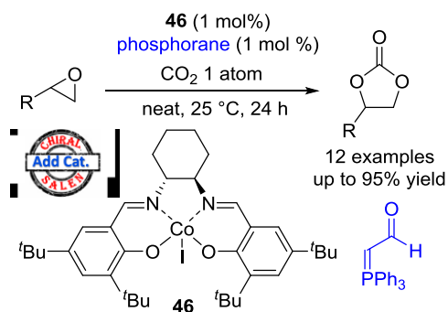
Scheme 60. Carbonate formation from CO 2 and epoxides with catalyst 46 and a phosphorane additive
