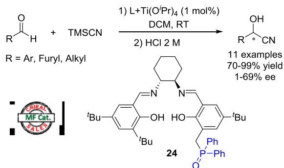
Scheme 28. Cyanosilylation of aldehydes with bifunctional (salen)Ti/TPPO catalyst 24 (unspecified absolute configuration)
