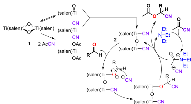
Scheme 3. Proposed mechanism for the enantioselective cyanation of aldehydes with 1 and Et 3 N (all intermediates are Ti IV species)
