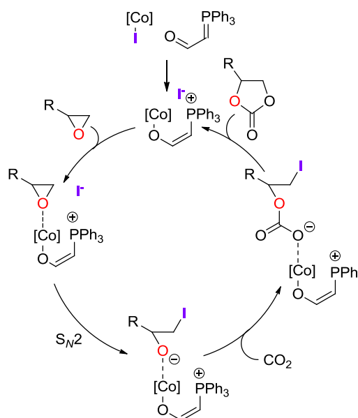
Scheme 61. Proposed mechanism for the catalytic synthesis of carbonates with 46 and a phosphorane additive
