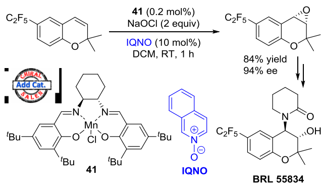
Scheme 52. Asymmetric epoxidation of a chromene derivative catalyzed by complex 41 with IQNO as an additive
