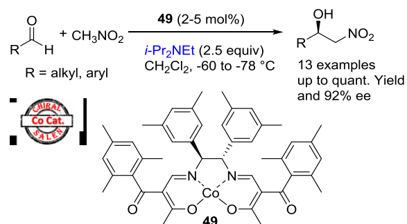
Scheme 64. Henry reaction catalysed by complex 49
