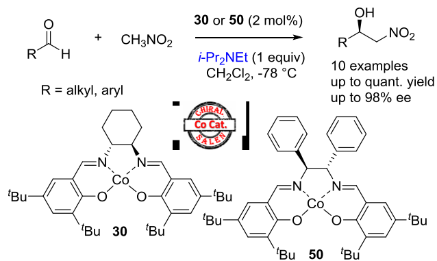
Scheme 65. Catalytic enantioselective Henry reaction with complexes 30 or 50 and DIPEA
