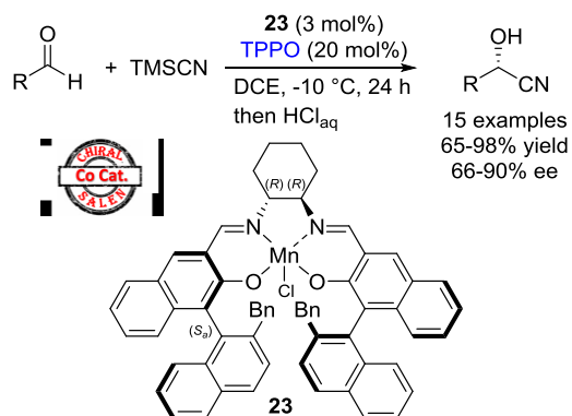
Scheme 27. Cyanosilylation of aldehydes catalyzed by salen complex 23 and TPPO
