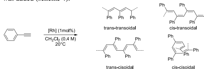
Scheme 4. Rhodium-catalyzed Polymerization of phenylacetylene leading to configurationally different poly(phenylacetylene) (PPA).
