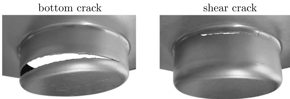
Fig. 2. Location of cracks observed experimentally in deep drawing experiments (after Gorji et al., 2016b). In the case of a blank-holder force of 200 kN, a shear crack appears for a blank size L between 133 mm and 150 mm while a bottom crack occurs for a blank size L above 150 mm.
