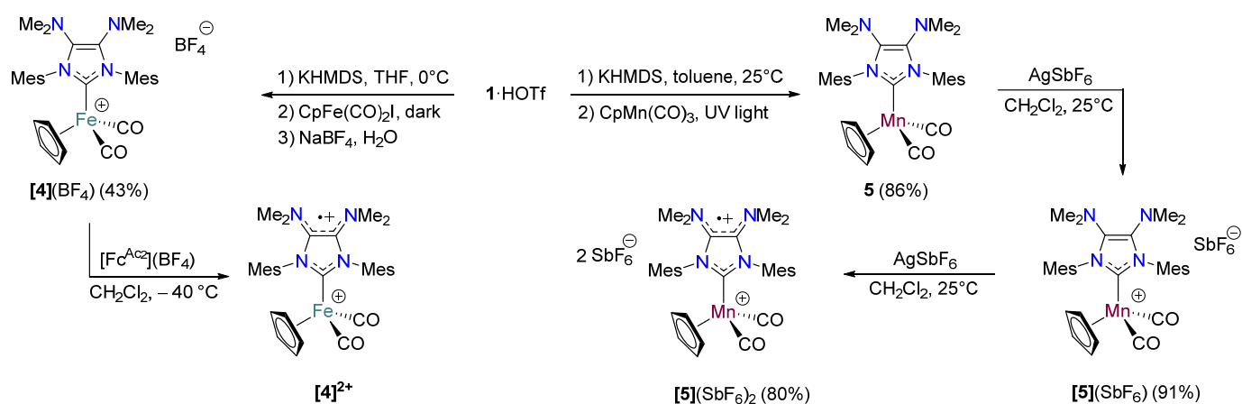
Scheme 1. Synthesis of the Fe(II) complex [4](BF 4 ), and chemical generation of the oxidized Fe(II) complex [4] 2+ (left). Synthesis of Mn(I) complex 5, and its stepwise oxidation to Mn(II) derivatives [5](SbF 6 ) and [5](SbF 6 ) 2 (right).
