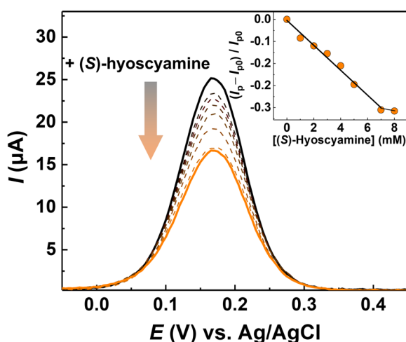
Fig. 4 DPV results of the MIP-AuNS electrode by adding ( S )-hyoscyamine in a phosphate buffer (100 mM, pH 7.0) containing K 3 Fe(CN) 6 (5 mM) and KCl (100 mM) at 25 °C. Inset represents the ratio of the peak current ( I p ) changes of the MIP-AuNS electrode. The terms I p0 and I p indicate the peak current before and after adding ( S )-hyoscyamine, respectively. [( S )-Hyoscyamine] = 0.0–8.0 mM.
