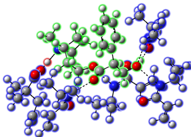
Fig. 2 The molecular complex (NIPAM:DMPA:( S )-hyoscyamine = 4:1:1) optimized by DFT calculation at the B3LYP (D3BJ)/def2SVP level with IEFPCM solvent model (solvent set as water).
