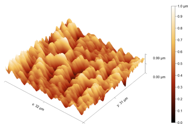
Fig. 3 FM-AFM image of the MIP-gold nanostructure (AuNS) attached extended-gate electrode.
