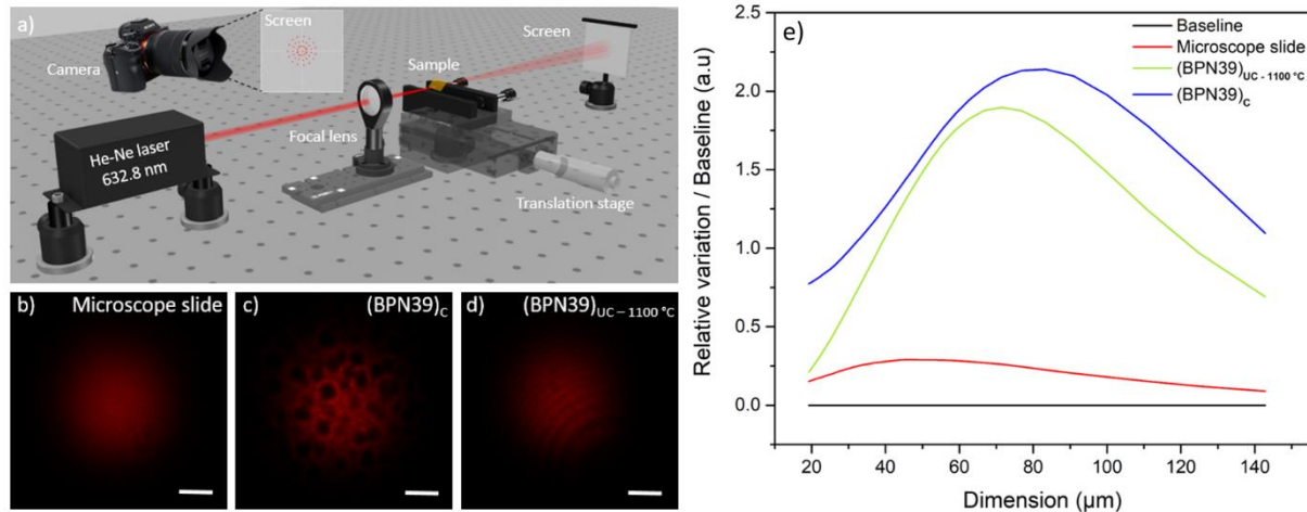
Fig 4. Shadowsopy imaging: a) Set-up of the experiment b) Micrograph of a Fischer microscope glass slide c) Micrograph of a casted sample (BPN39) c d) Micrograph of an uncasted sample (BPN39) UC-1100°C (scale bar = 2 cm) e) Relative variation of the striae magnitude as a function of their size
