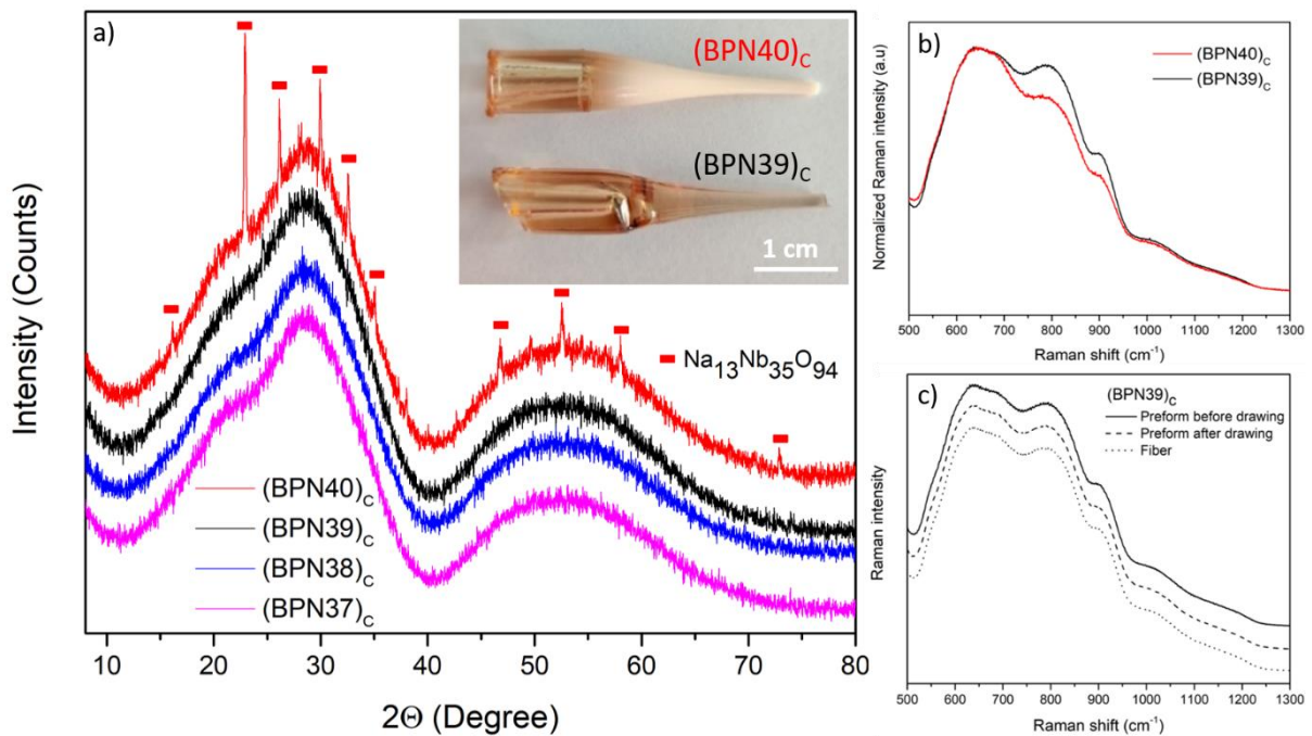
Fig 2. a) XRD pattern on BPN fibers after drawing and a photo of the preform neck-down of BNP39 and BPN40 is shown in inset. b) Raman spectrum on the neck down area, on both BPN39 and BPN40 and c) Raman spectrum of a BPN39, on the preform before the drawing process after the drawing process and on the fiber
